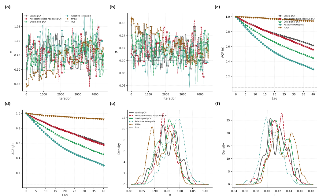
Figure 7. Sampling diagnostics for the CQNLSE inverse problem across all five methods. (a) Trace plots of \alpha ; (b) trace plots of \beta ; (c) autocorrelation functions for \alpha ; (d) autocorrelation functions for \beta ; and (e,f) posterior marginal densities. The AM showed the fastest decorrelation, while the MALA exhibited poor mixing.
