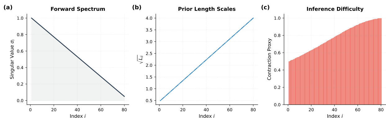
Figure 2. Problem setup for the linear-Gaussian benchmarks. (a) Singular value spectrum of the forward operator showing controlled decay. (b) Prior length scales across dimensions. (c) Inference difficulty as measured by the posterior contraction ratio across regimes.
