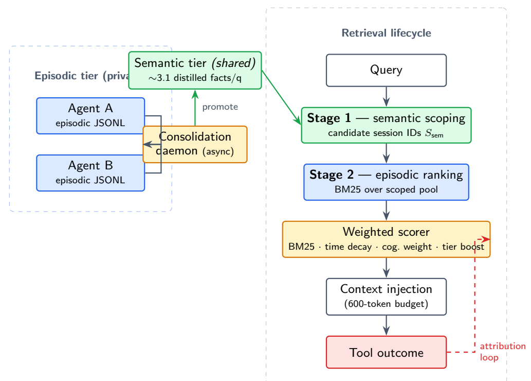
Figure 1. Graphical overview of MEMTIER. Left: the tiered architecture (episodic store, semantic tier, and a multi-signal scoring scaffold over two-stage scoping). Right: the memory components studied—session-level injection, drop-one evidence-coverage attribution, and typed consolidation. Detailed component diagrams appear in Figure 2 and Section 3. As our ablation shows (Section 4), the scoring scaffold operates as a BM25 pass-through in this regime. We study these components as related diagnostics rather than a single validated pipeline.
