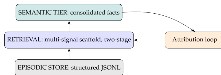
Figure 3. The MEMTIER architecture. Episodic entries are scored by the multi-signal retrieval scaffold using two-stage semantic→episodic scoping; a consolidation daemon promotes high-value episodes to a project-shared semantic tier; an attribution loop updates per-entry cognitive weight from tool outcomes. Section 4 shows the scaffold reduces to BM25 top- k in the evaluated regime.
