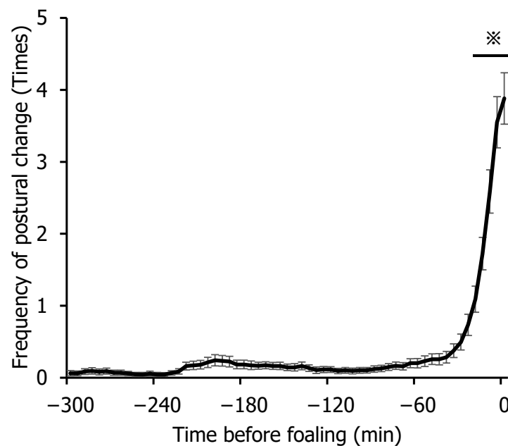
Figure 3. Temporal changes in posture change frequency during the 5 h preceding foaling. Data are presented as the mean \pm SE. Time 0 represents the moment of foaling. Meanwhile, asterisks indicate significant differences compared with the value at -300 min ( p < 0.05 ).
