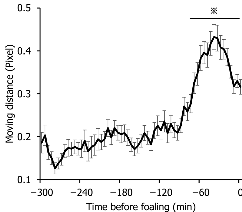
Figure 1. Temporal changes in locomotor activity during the 5 h preceding foaling. Data are presented as the mean \pm standard error (SE). Time 0 represents the moment of foaling. Meanwhile, asterisks indicate significant differences compared with the value at -300 min ( p < 0.05 ). Locomotor activity was expressed as moving distance in pixel units derived from centroid displacement in thermal images. Pixel-based movement represents relative displacement within the image frame and provides a consistent index of locomotor activity across individuals.
