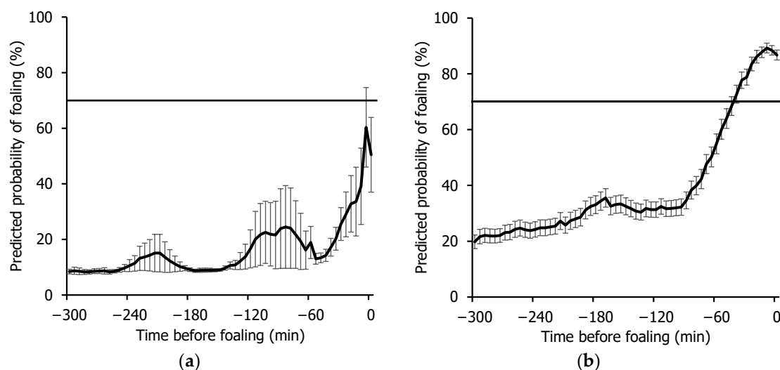
Figure 5. Temporal changes in the predicted foaling probability using model 2 during the 5 h preceding foaling. (a) Predicted foaling probability in the four mares that were not detected prior to foaling. In these cases, the probability gradually increased but did not exceed the predefined detection threshold of 70%. (b) Predicted foaling probability in the 109 mares that were successfully detected before foaling. In all detected cases, the probability exceeded the 70% threshold prior to foaling. Time 0 represents the moment of foaling. Meanwhile, the dashed horizontal line indicates the predefined detection threshold (70%).
