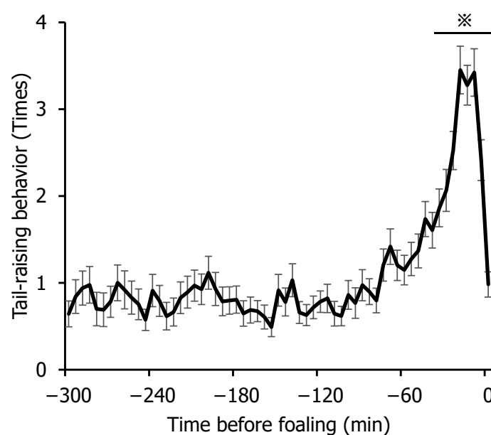
Figure 4. Temporal changes in tail-raising behavior during the 5 h preceding foaling. Data are presented as the mean \pm SE. Time 0 represents the moment of foaling. Meanwhile, asterisks indicate significant differences compared with the value at -300 min ( p < 0.05 ).
