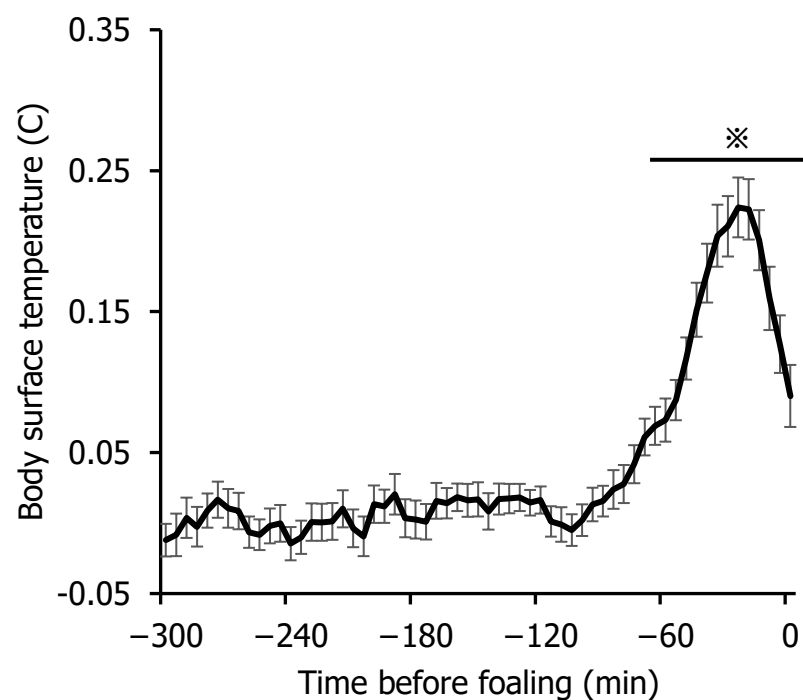
Figure 2. Temporal changes in surface temperature measured by thermal imaging during the 5 h preceding foaling. Values represent the mean body surface temperature difference between the segmented mare region and ambient temperature. Data are presented as the mean \pm SE. Time 0 represents the moment of foaling. Meanwhile, asterisks indicate significant differences compared with the value at -300 min ( p < 0.05 ).
