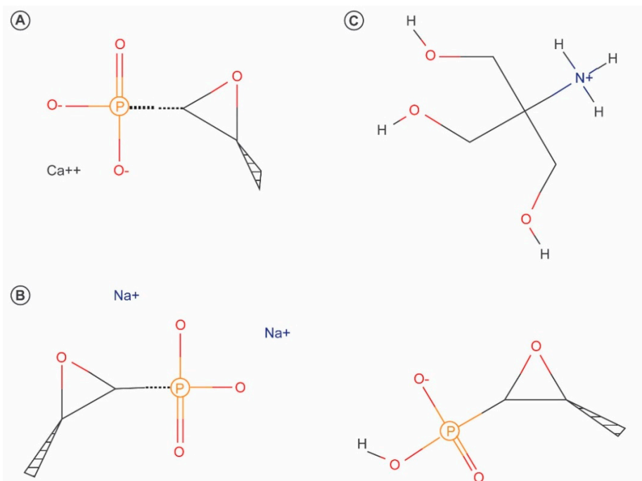
Figure 2. Chemical structures of fosfomycin calcium (A), fosfomycin disodium (B) and fosfomycin tromethamine (C).
