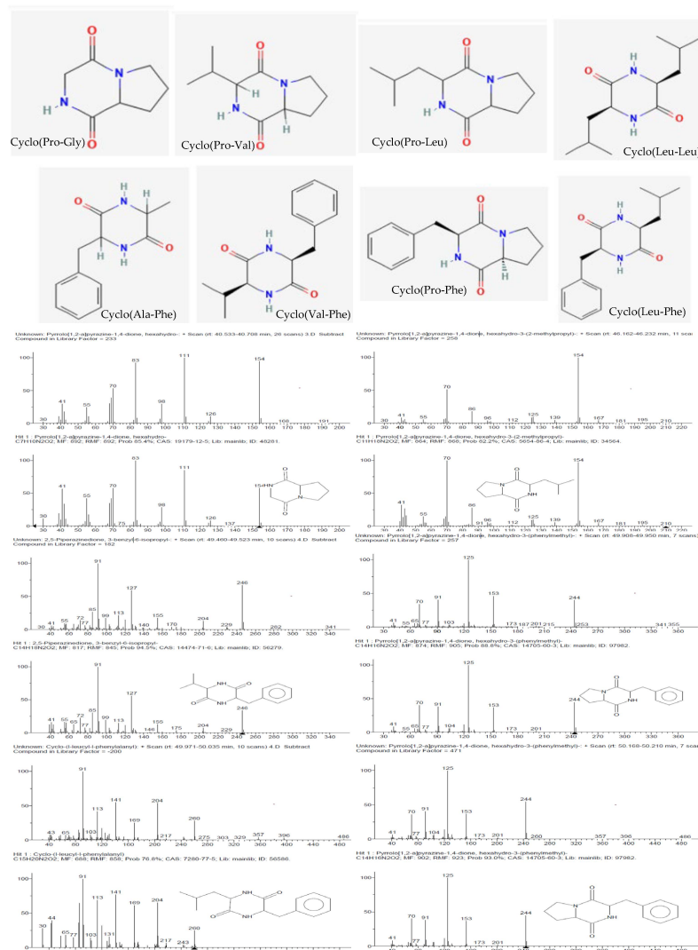
Figure 4. Structures (obtained from PubChem) and mass spectra of the 2,5-diketopiperazines (identified by comparison with the mass spectra in the NIST 11 library) present in the ECBp14, CELr30, CEPp48, and CEPp49 extracts.
