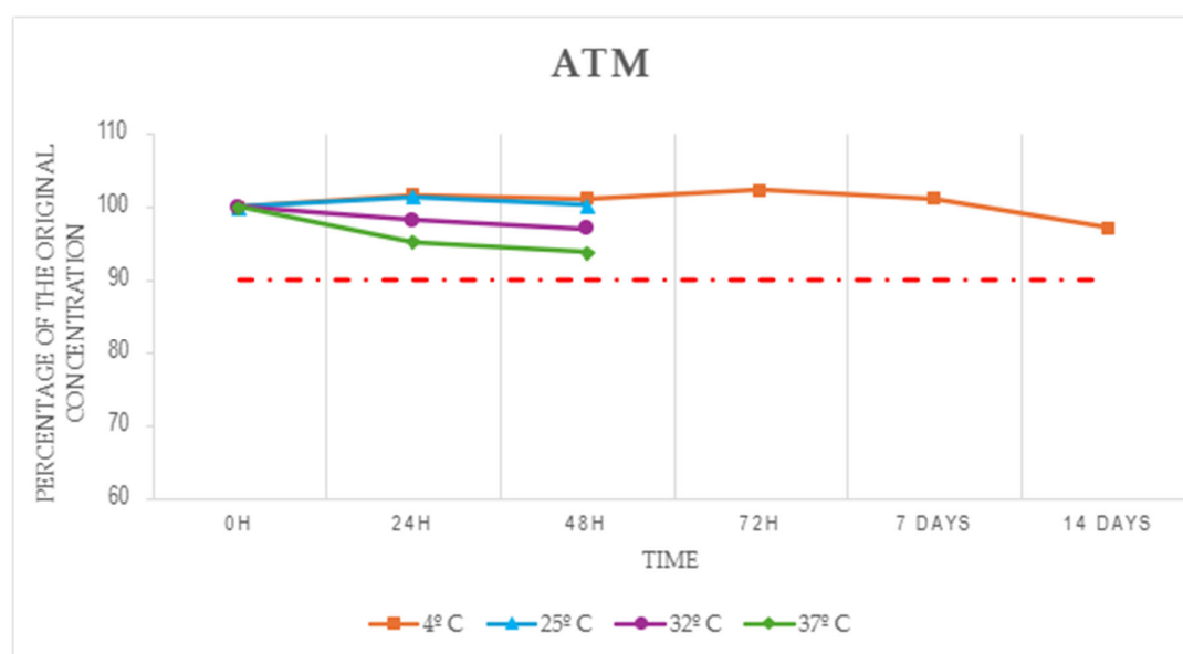
Figure 1. Stability of ATM (aztreonam) expressed as mean percentage of original concentration over time at 4 °C, 25 °C, 32 °C, and 37 °C.
