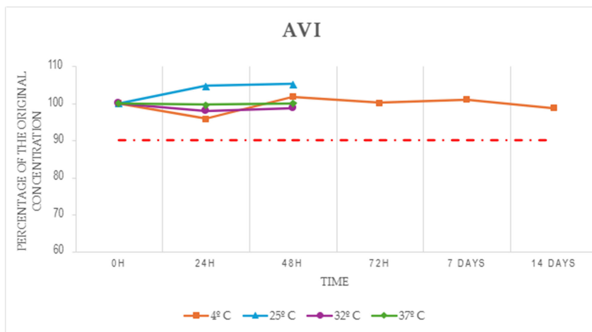
Figure 2. Stability of AVI (avibactam) expressed as mean percentage of original concentration over time at 4 °C, 25 °C, 32 °C, and 37 °C.
