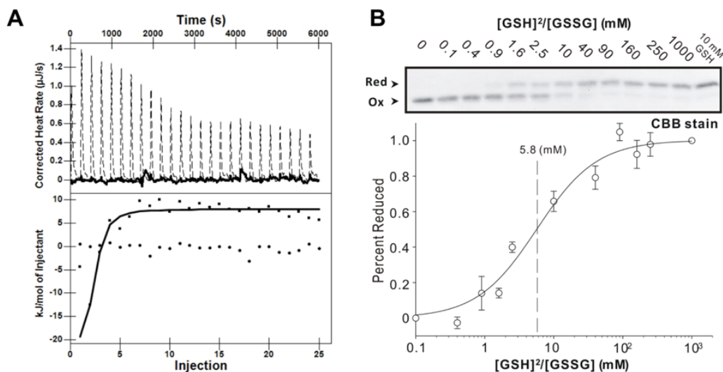
Figure 3. AtAPR1 redox domain possesses glutaredoxin activity. (A) Isothermal titration calorimetric thermogram (top) and isotherm (bottom) for the glutathionylation of the AtAPR1 redox domain. The dotted line in the thermogram is the adjusted calorimetric baseline. The solid line in the isotherm was obtained from nonlinear least-squares regression to both the OneSites and the Exchange model (the regression lines from the two algorithms coincide). (B) Determination of the equilibrium constant of the AtAPR1 redox domain with glutathione at pH 7.0 and 25 °C. (top) After incubation with different [GSH] 2 /[GSSG] ratios, the free sulfhydryl groups of the cysteine residues were modified with use of AMS (Bottom). A fraction of the reduced AtAPR1 redox domain was used to measure the redox equilibrium constant of the AtAPR1 redox domain. The apparent equilibrium constant between the AtAPR1 redox domain and glutathione was calculated by nonlinear least-squares fitting of the data in the upper column.
