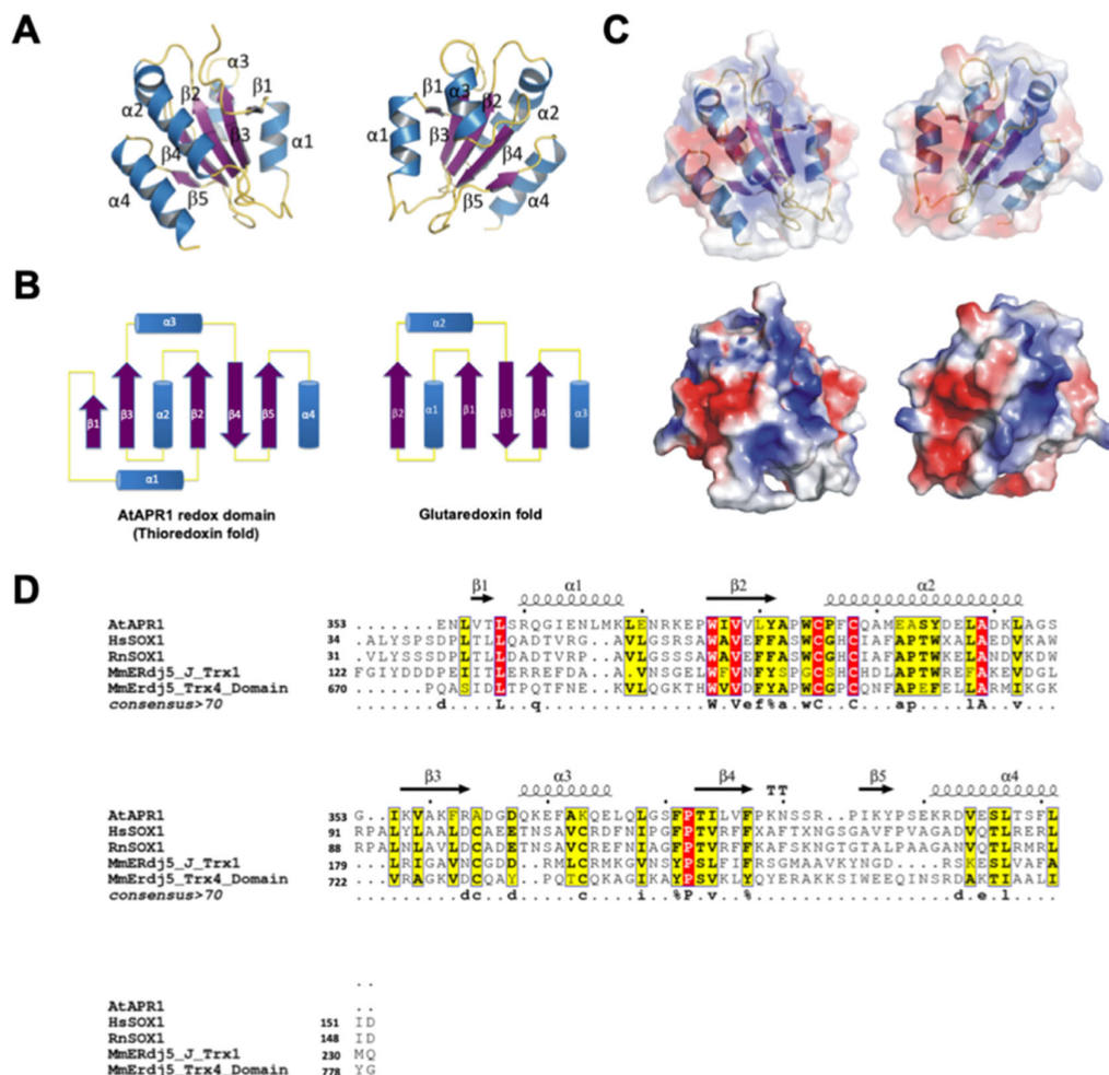
Figure 2. Crystal structure of the C-terminal redox domain of AtAPR1. (A) Structure of the AtAPR1 redox domain displays a typical thioredoxin fold with a central five-stranded \beta -sheet ( \beta 1– \beta 5) and four flanking \alpha -helices ( \alpha 1– \alpha 4). Helices, strands, and loops are shown in blue, purple, and yellow, respectively. (B) Topology diagram of the AtAPR1 redox domain and glutaredoxin fold. (C) The electrostatic surface potentials mapped with red patches and blue patches represented as negative and positive charge, respectively. (D) Structure-based sequence alignment of the AtAPR1 redox domain with other structural homologs. Selected proteins shown in alignment are human sulfhydryl oxidase 1 (hsSOX1; PDB code: 3Q6O), rat sulfhydryl oxidase 1 (RnSOX1; PDB code: 4P2L), mouse ER-resident protein disulfide reductase (MmERdj5) J-Trx1 fragment (PDB code: 3APQ), and mouse ER-resident protein disulfide reductase (MmERdj5) TRX4 domain (PDB code: 3APS). Identical residues are in white and the frame is in red. Amino acids with similarity score > 0.7 are framed in yellow. Secondary structure of the AtAPR1 redox domain is drawn above the alignment with arrows as sheets and strings as helices.
