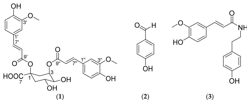
Figure 1. Chemical structures of compounds 1 to 3 ; ( 1 ) 1,3-di- O - trans -feruloyl-(-)-quinic acid, ( 2 ) p -hydroxybenzaldehyde, and ( 3 ) N - trans -feruloyltyramine.
