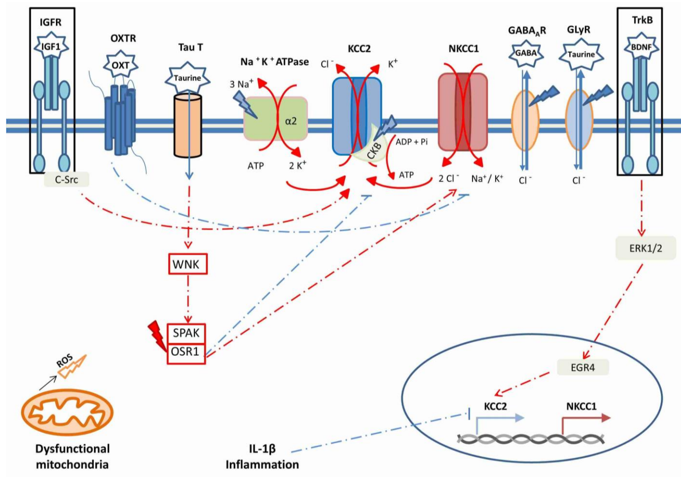
Figure 2. The main factors modulating KCC2 and NKCC1 synthesis and activity, in relation with anomalies described in neurological and neurodevelopmental disorders. Oxidative stress/ROS is symbolized by lightning bolts; blue bolts indicate a loss-of-function effect, red bolts indicate a gain-of-function effect. The boxes surrounding IGFR and TrkB indicate that IGF-1 and BDNF signaling are both decreased in ASD and in other neurodevelopmental disorders.
