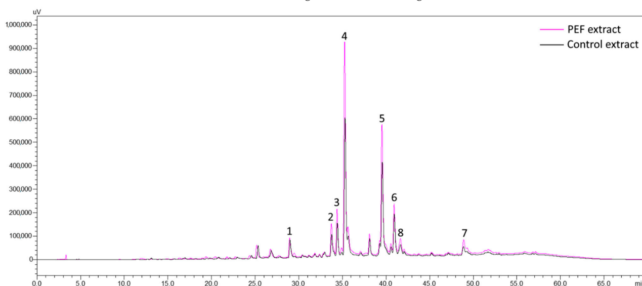
Figure 2. Overlay of chromatograms of PEF and control extracts with t_{\text{pulse}} 10 \mu\text{s} and T 1000 \mu\text{s} . Peak 1: Luteolin diglucoside; Peak 2: Quercetin-3- O -rutinoside; Peak 3: Luteolin rutinoside; Peak 4: Luteolin-7- O -glucoside; Peak 5: Apigenin-7- O -rutinoside; Peak 6: Luteolin-3'- O -glucoside; Peak 7: Luteolin aglycone; Peak 8: Oleuropein.
