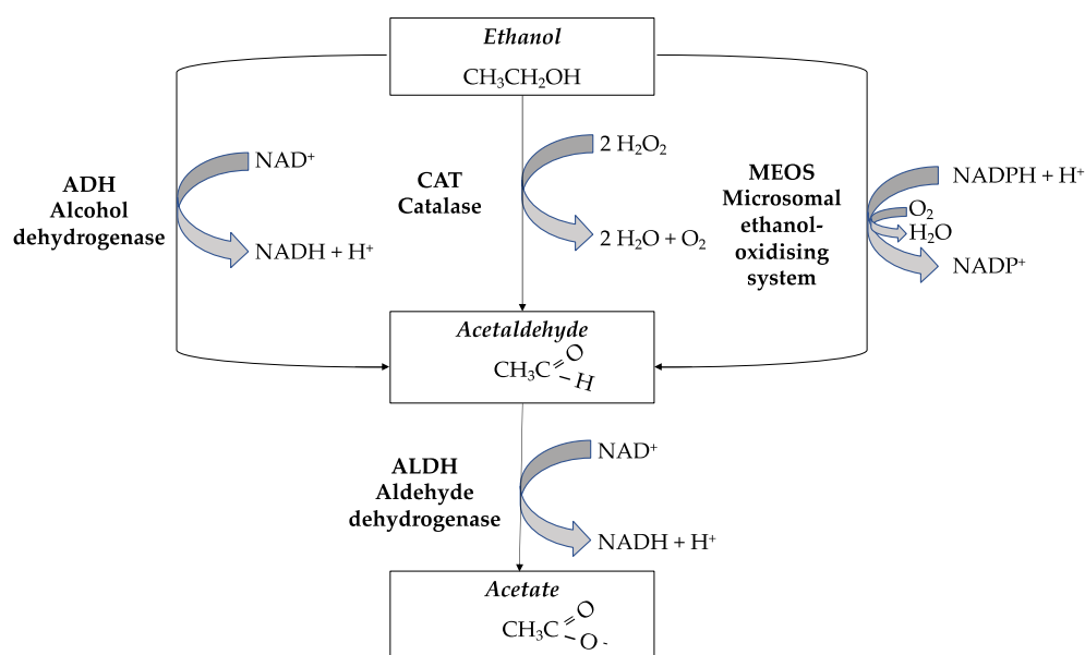
Figure 1. Ethanol metabolism.
