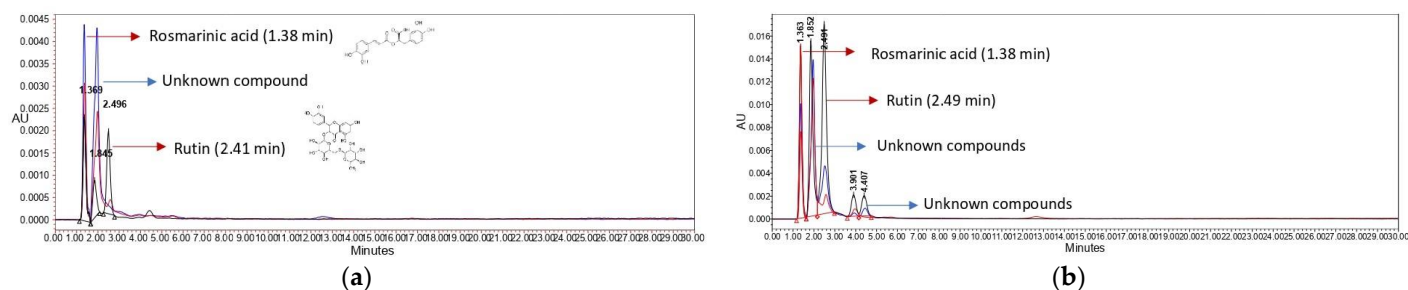
Figure 2. Chromatographic profile of the Gypsophila taxa: (a) stem extracts and (b) leaf extracts of G. eriocalyx (red), G. germanicopolitana (blue), and G. simonii (black).
