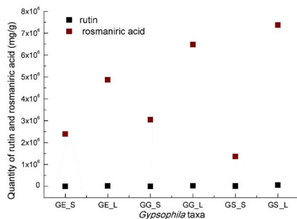
Figure 3. Quantification levels of rosmarinic acid and rutin in three different extracts of Gypsophila taxa: G. eriocalyx stem (GE_S), G. eriocalyx leaf (GE_L), G. germanicopolitana stem (GG_S), G. germanicopolitana leaf (GG_L), G. simonii stem (GS_S), and G. simonii leaf (GS_L).
