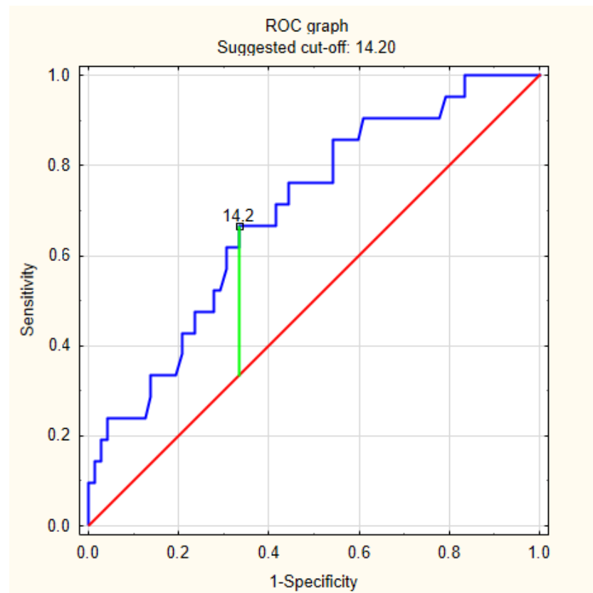
Figure 2. ROC curve of discrimination of CAD-RADS \geq 3 based on AH1 (/h) values in the study group.
