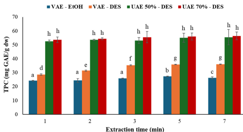
Figure 1. Total phenolic content (TPC) as a function of extraction solvent, extraction technique, and extraction time. Conditions: vortex-assisted extraction with 70% ethanol (VAE-EtOH), vortex-assisted extraction with DES (VAE-DES), and ultrasound-assisted extraction with DES at 50% and 70% amplitude (UAE-DES 50% and UAE-DES 70%). Bars represent mean \pm SD ( n = 3 ). Different letters indicate significant differences according to Tukey's HSD test ( p < 0.05 ). TPC is expressed as mg GAE/g dw.
