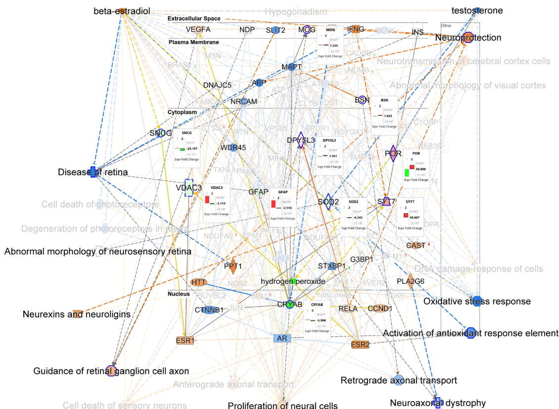
Figure 5. Focus view of the interaction network shown in Figure 4, generated by IPA®'s PE among the selected DEPs (SOD2, VDAC3, CRYAB, GFAP, SNCG, BSN, SYT7, DPYSL3, POR, and MOG), E2, T, and their respective nuclear receptors (ESRs and AR), and key elements of OS and neuroprotective response pathways, with quantitative proteomic data (with and without DHED treatment) overlaid via IPA®'s Data Overlay platform. Line annotations: orange—activation/increase; blue—inhibition/decrease; yellow dashed—effect cannot be predicted; grey—direct or indirect relationship without predicted directionality (solid: direct; dashed: indirect relationship). Node color: red—upregulation; green—downregulation; shade intensity reflects the magnitude of change in protein expression. Inset: protein expression for the ORX group (1st bar) and DHED-treated group (2nd bar); the naïve group is not shown, as it serves as the fold-change baseline. Abbreviations are listed in Table S5b.
