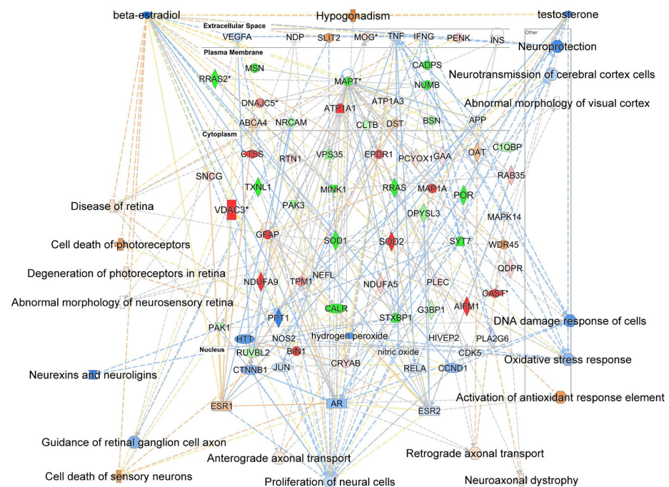
Figure 4. Interaction network generated by IPA®'s PE among the ORX-impacted DEPs in the VC (SOD2, VDAC3, CRYAB, GFAP, SNCG, BSN, SYT7, DPYSL3, POR, and MOG), incorporating E2, T, and their respective nuclear receptors (ESR1, ESR2, and AR), as well as components of the OS response and neurodegenerative pathways. Line annotations: blue solid/dashed line—inhibition/decrease; orange dashed line—activation/increase; yellow dashed line—effect cannot be predicted; grey solid/dashed line—direct or indirect relationship, respectively, without predicted directionality. Node color: red—upregulated; green—downregulated; shade intensity reflects the magnitude of change in protein expression. Protein name abbreviations are listed in Table S5b, * denotes multiple isoforms identified by IPA®.
