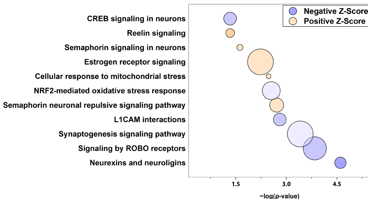
Figure 3. ORX-regulated proteins involved in top canonical pathways associated with the OS response in the male BN rat VC. Bubble size indicates the number of proteins overlapping with each pathway. Orange and blue colors represent predicted activation and inhibition, respectively.
