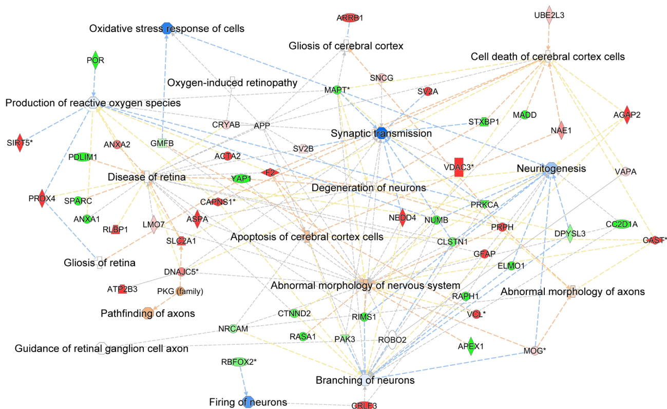
Figure 2. IPA®-generated network of ORX-induced proteome alterations associated with OS and neurodegenerative functions in the male BN rat VC. The network was constructed based on DEPs identified between naïve (intact) and ORX animals, with IPA® predicting activation or inhibition of disease- and function-related networks. Line annotations: orange solid/dashed—predicted activation; blue solid/dashed—predicted inhibition; yellow dashed—effect cannot be predicted; grey solid/dashed—direct/indirect relationship without predicted directionality. Node color reflects the direction and magnitude of change: red indicates upregulation, and green indicates downregulation in the dataset, with shade intensity corresponding to the magnitude of change in protein expression. Red and green reflect actual measurements, while orange and blue reflect IPA®-predicted activation/inhibition. Edge lines represent known protein–protein interactions according to IPA®'s Knowledge Base. The abbreviated protein names are listed in Table S5a, * denotes multiple isoforms identified by IPA®.
