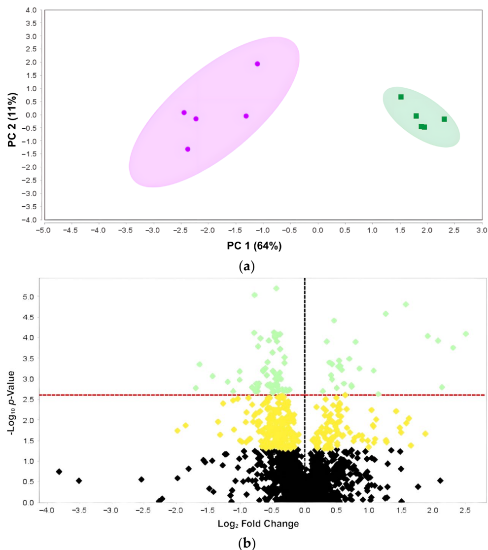
Figure 1. Scaffold-based proteomic analyses of the male BN rat VC. (a) PCA plot illustrates the separation between the VC proteome of the naïve (intact, green) and ORX (magenta) groups. (b) Volcano plot depicting DEPs between the naïve (intact) and ORX groups. Green—significant after BH multiple testing correction; yellow—significant before BH correction; black—not significant. Left panel represents downregulated proteins, while the right panel represents upregulated proteins.
