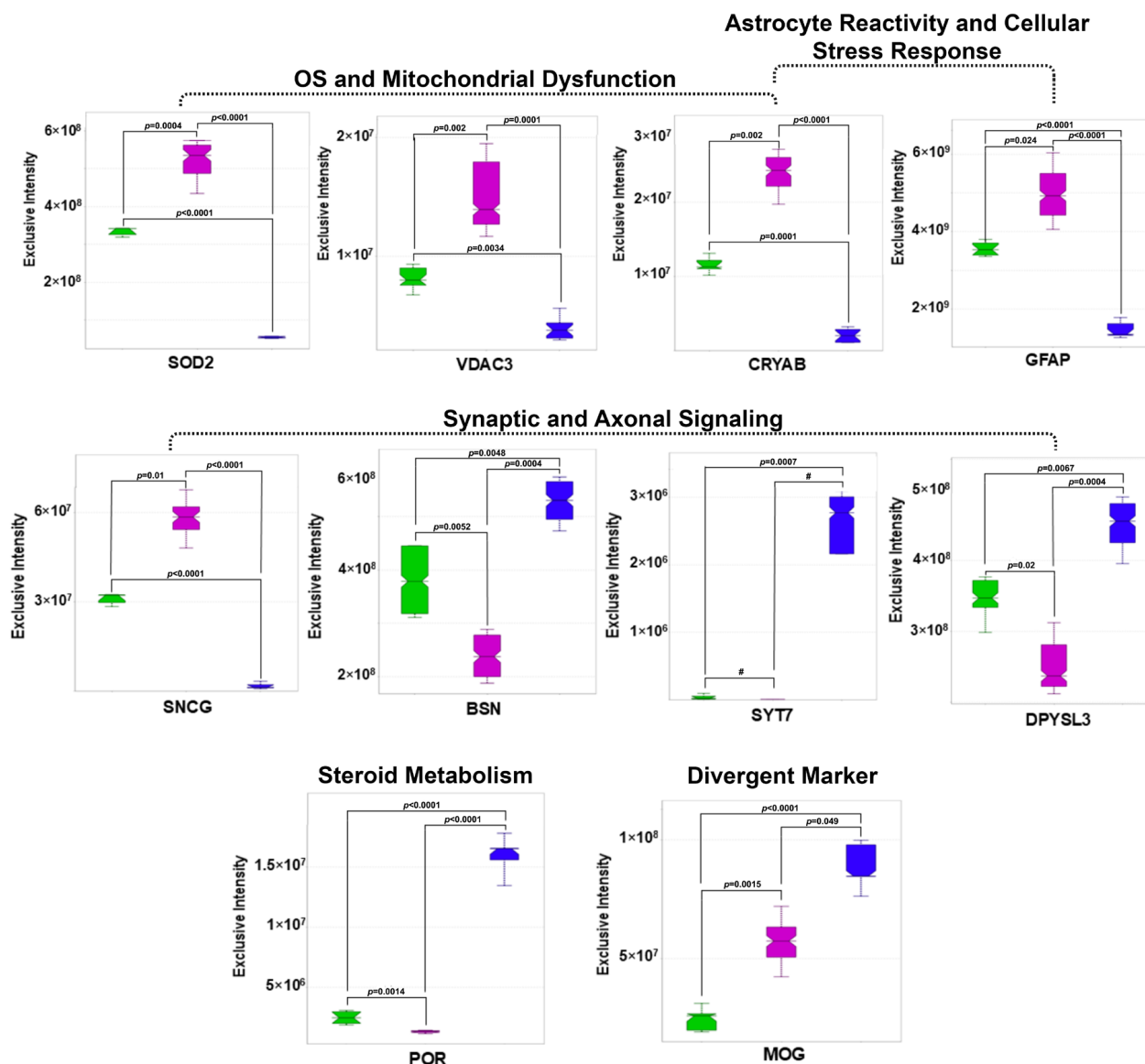
Figure 6. Scaffold DIA-based quantitative survey of key DEPs from Figures 4 and 5, predicted by IPA ® to be involved in neuroprotection. Box plots: green—naïve (intact); magenta—vehicle; blue—DHED. Protein descriptions and transitions used for quantitation are in Tables S6a and S6b, respectively; raw intensities for all samples are listed in Table S6c. One-way ANOVA with post hoc Tukey–Kramer tests ( n = 5/\text{group} ) showed statistically significant differences between all group pairs for all listed proteins; p -values are displayed on the chart; #—not tested).
