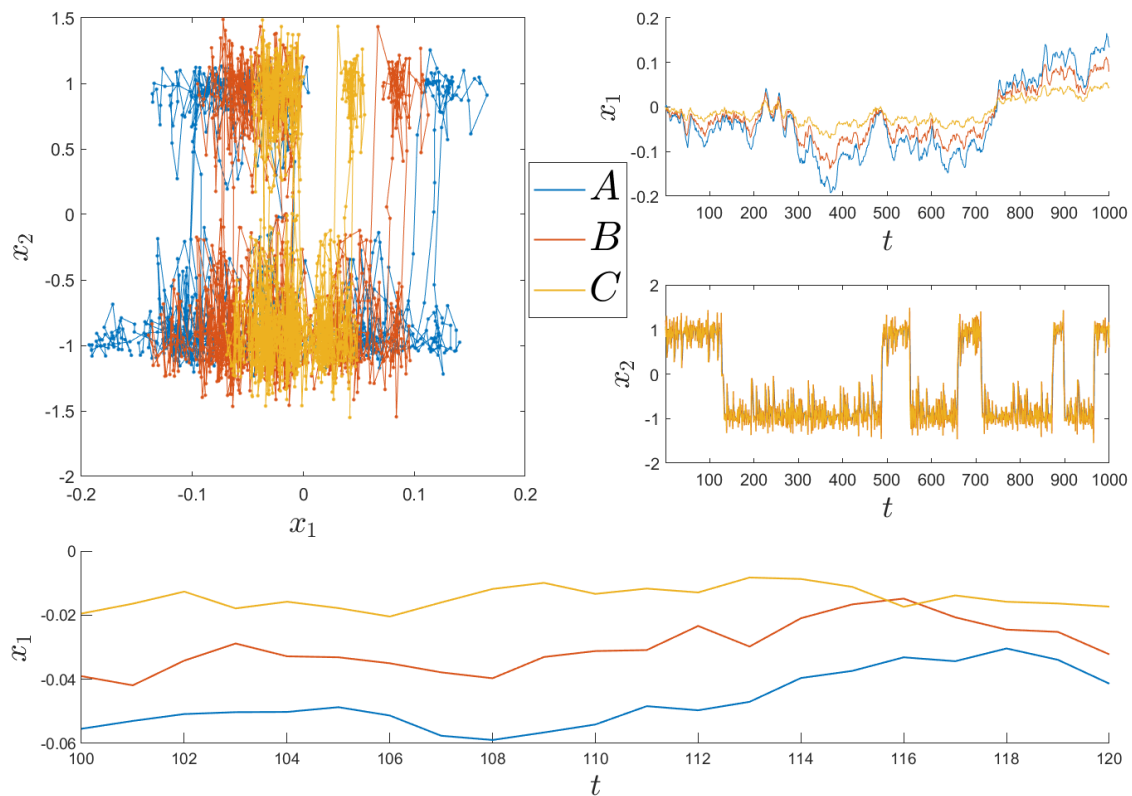
Figure 5. Realisation of the system described by Equation (22). A in blue, B in orange, C in yellow. One can see the metastable behaviour in the x_2 -coordinate in C , which the other processes emulate. Parameters: \alpha = 5 , \sigma_C = \text{diag}((0.01, 0.05)) , \sigma_B = \sigma_A = 0.01 .
