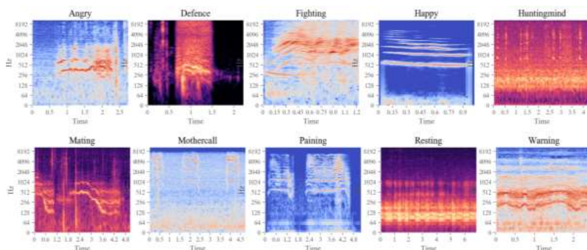
Figure 4. The sample in Figure 2 transformed to log power spectrogram.
