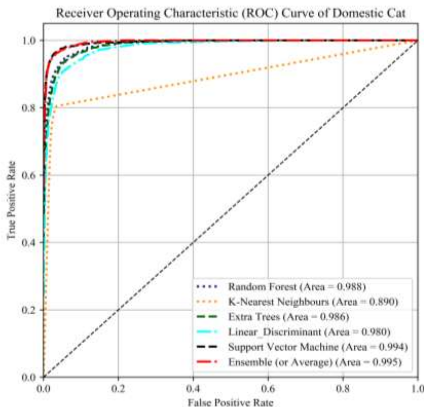
Figure 8. ROC curves of the various classifiers with 3x_Aug datasets using CDBN features. Each curve is represented by a unique color and corresponding AUC score is given in parentheses.
