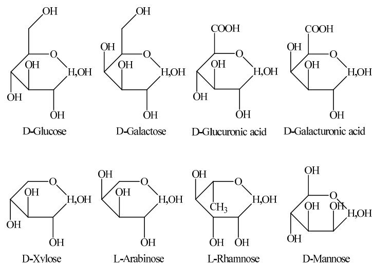
Figure 1. The monosaccharide structure of Astragalus polysaccharides.
