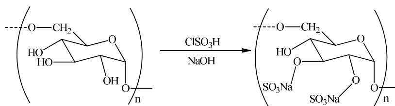
Figure 2. The reaction of APS sulfate by the chlorosulfonic acid–pyridine (CSA–Pyr) method [54].
