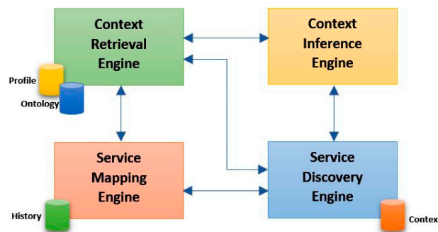
Figure 9. Distributed Context Management Module.
