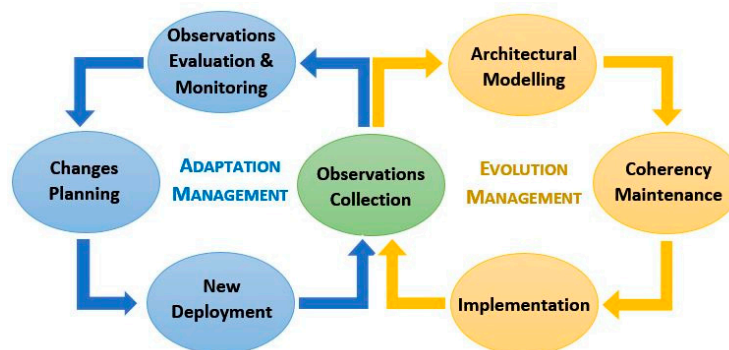
Figure 13. Mechanisms of self-adaptation module.
