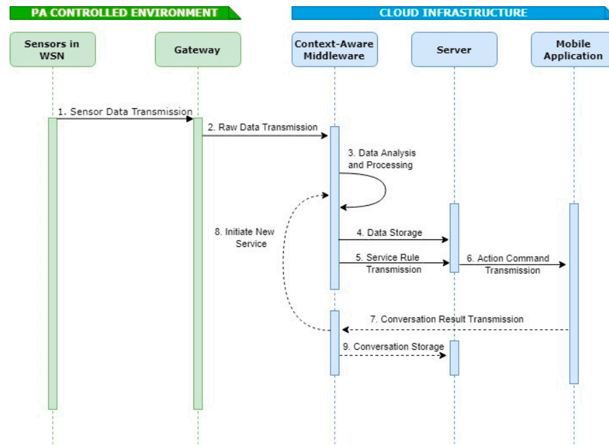
Figure 18. Sequence Diagram for Automated Context-aware Service.
