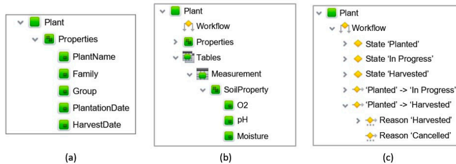
Figure 12. Indicative entity (a) properties, (b) table and (c) workflow.
