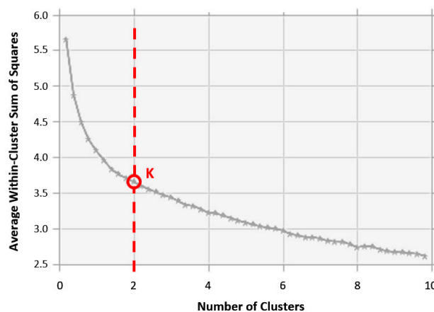
Figure 25. Elbow evaluation method for K-means clustering.
