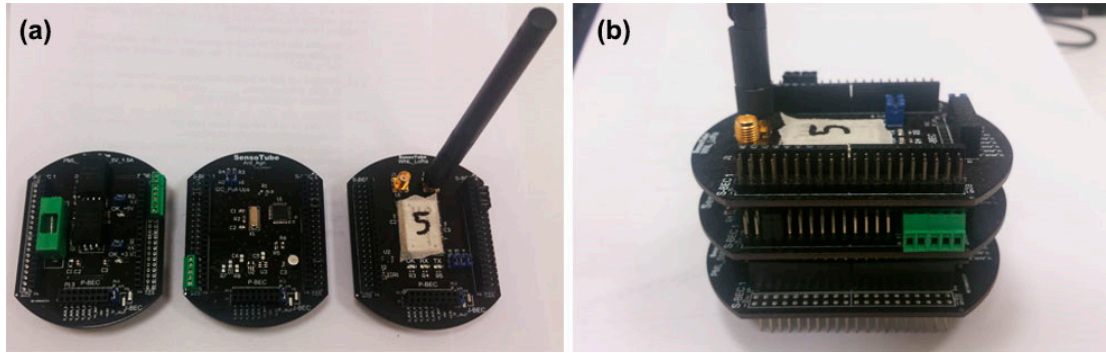
Figure 15. Wireless sensor hardware using the “SensoTube” open architecture: (a) Shields for i) LoRa wireless connectivity, ii) data acquisition and control and iii) energy management; (b) The three shields in a complete wireless node.
