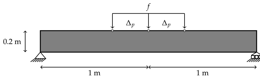
Figure 2. The various forces with respect to the location in three-point bending specimen.
