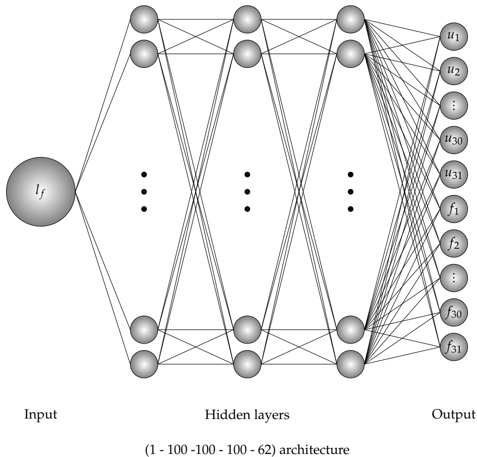
Figure 3. Deep neural network architecture for various location forces problem.
