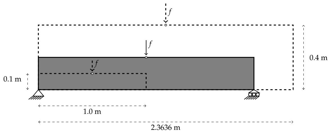
Figure 6. The various dimension for three-point bending specimen.
