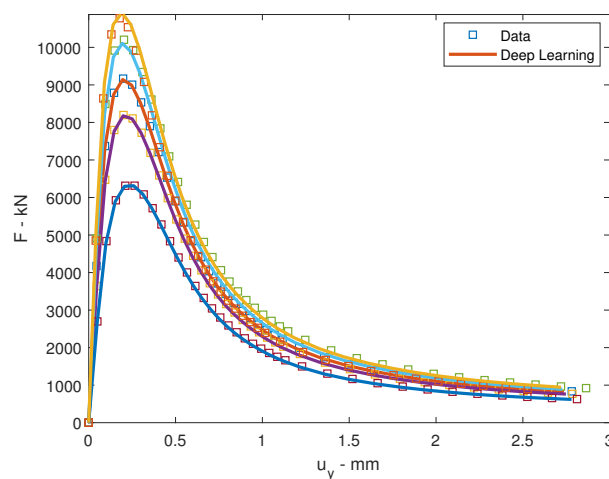
Figure 16. The testing of loading deflection curves for L-hape problem.
