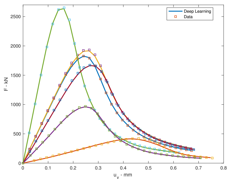
Figure 9. The testing of loading deflection curves for dimensional problem.
