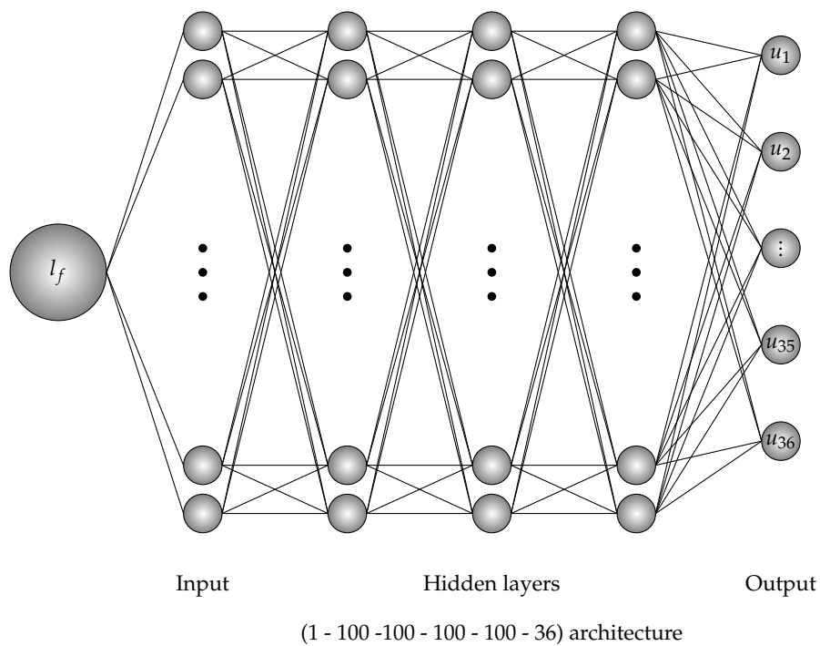
Figure 14. Deep neural network architecture for force locations problem of the L-shape specimen.
