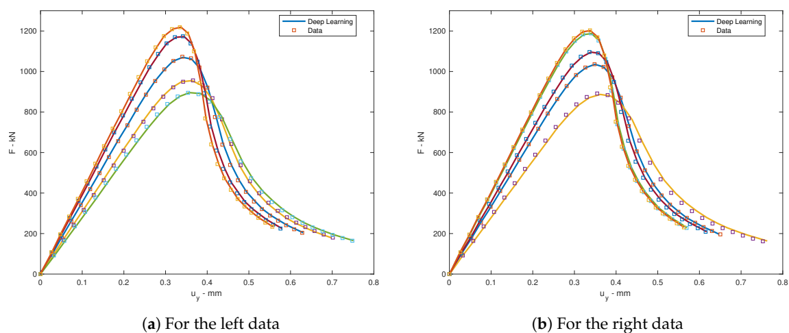
Figure 5. The testing of loading deflection curves for location-force problem.
