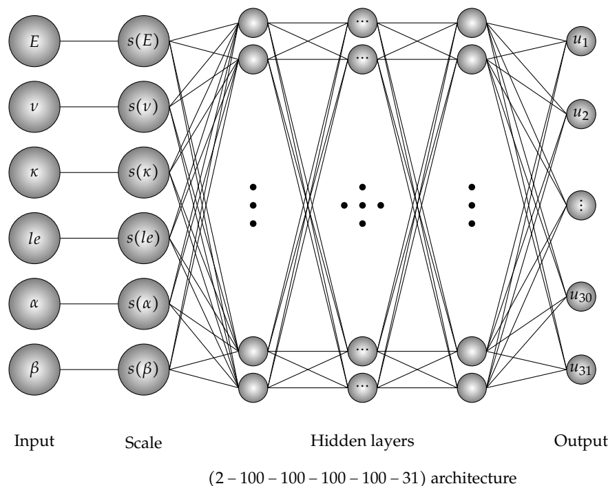
Figure 10. Deep neural network architecture for material parameter problem of the three-point bending specimen.
