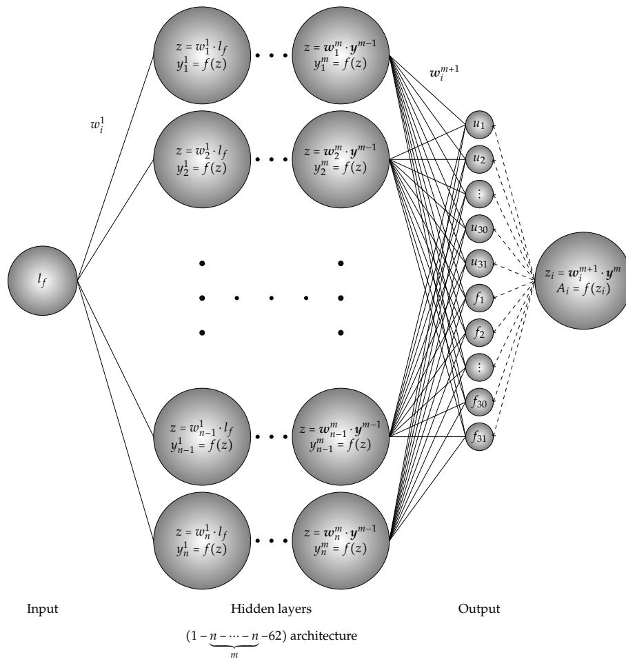
Figure 1. Activation function role in deep neural network.
