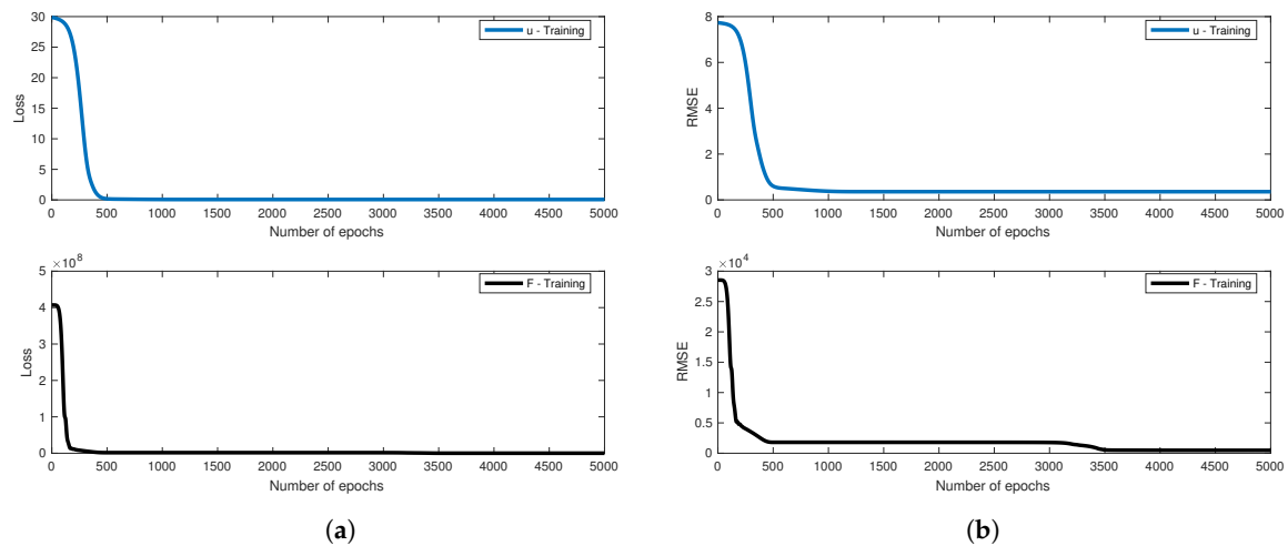
Figure 15. The training process for shear force problem in the L-hape specimen. (a) Mini-batch loss for L-shape shear force training process; (b) RMSE for L-hape shear force training process.
