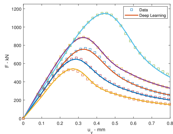
Figure 12. The testing of loading deflection curves for material problem.
