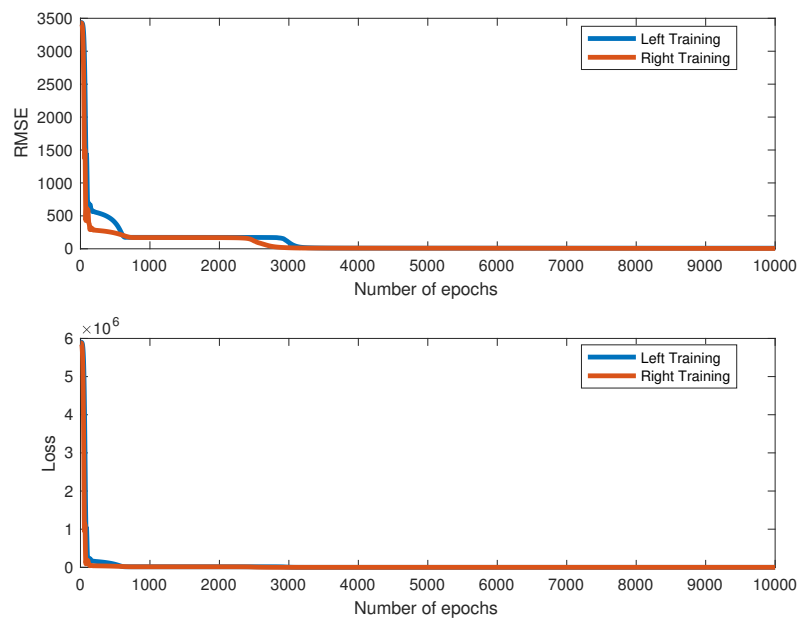
Figure 4. The training process for location-force data in three-point bending specimen.
