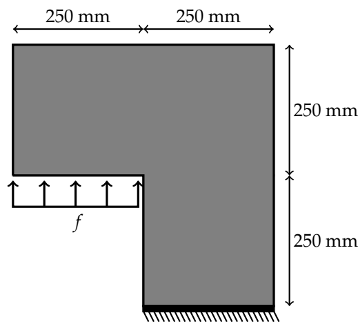
Figure 13. The various forces with respect to the location in L-shape specimen.
