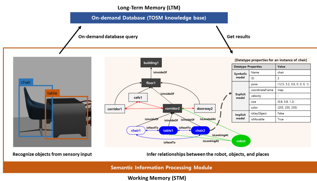
Figure 4. Semantic information processing module.
