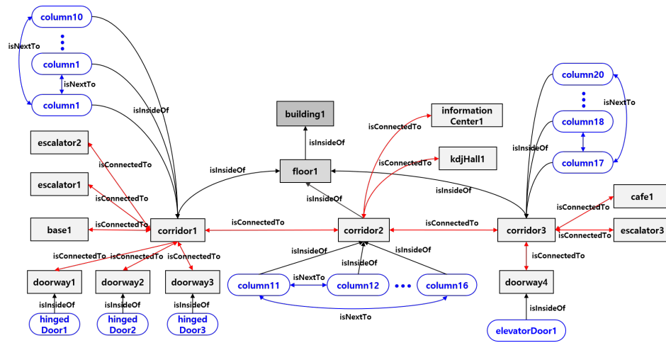
Figure 11. The TOSM-based database for experiments.
