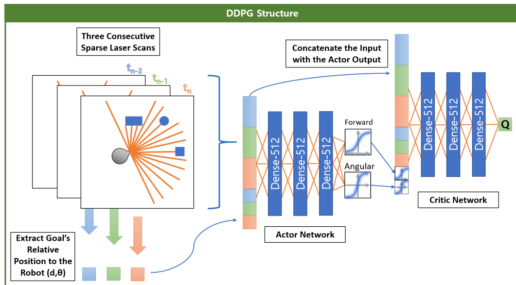
Figure 9. The Deep Deterministic Policy Gradients (DDPG) structure used to approximate an autonomous navigation policy.
