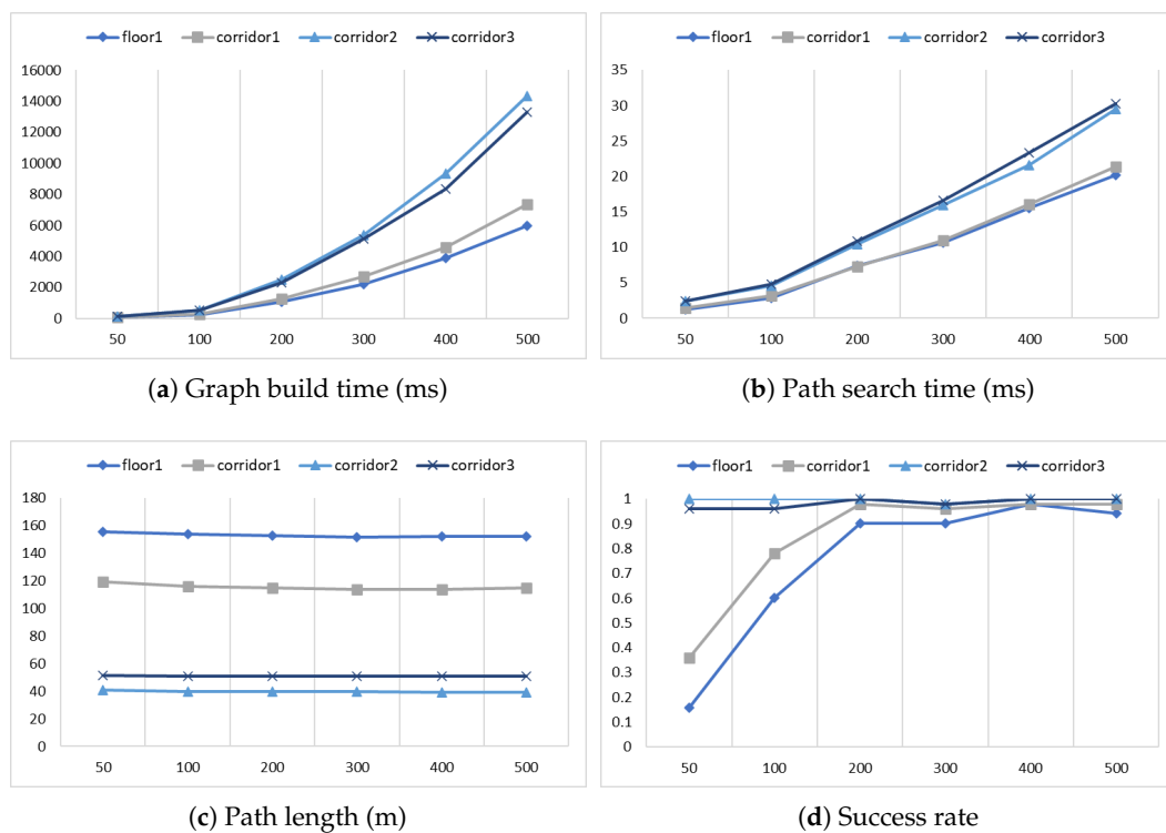
Figure 13. Influence of the number of samples (x-axis) on the PRM algorithm.
