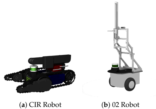
Figure 6. The CIR robot is equipped with a continuous track and extension arms, enabling going up and downstairs. The O2 robot is equipped with sensors and manipulators that allow elevator operation.
