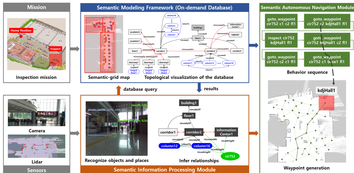
Figure 12. The TOSM-based autonomous navigation framework sequence diagram.
