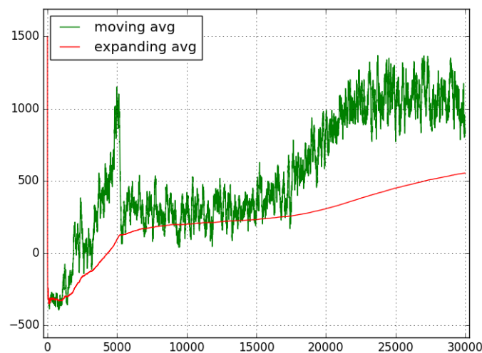
Figure 14. Reward obtained by the robot on each training episode. The line in green represents a moving average using a 100 episodes window. The line in red shows the cumulative average until the current episode.
