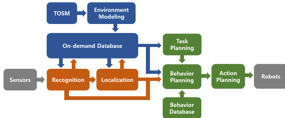
Figure 1. The proposed framework consists of semantic modeling framework (SMF) (blue blocks), semantic information processing (SIP) module (orange blocks), and semantic autonomous navigation (SAN) module (green blocks).
