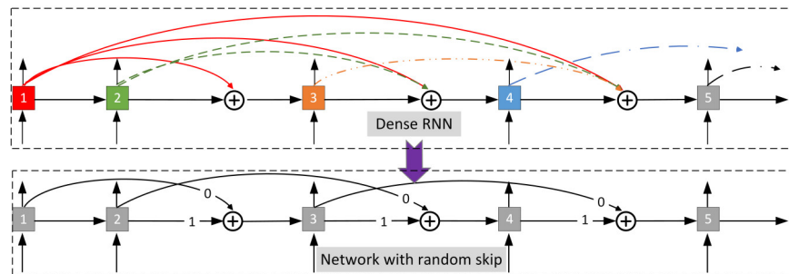
Figure 1. The framework of our proposed model. RNN: Recurrent neural network.
