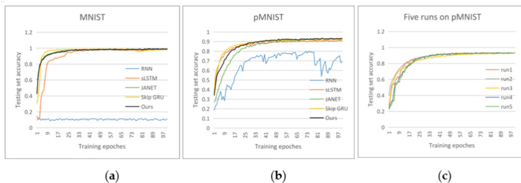
Figure 2. The change in test accuracy with training epochs. (a) accuracy on the MNIST, (b) accuracy on the pMNIST, (c) accuracy over five runs on the pMNIST.
