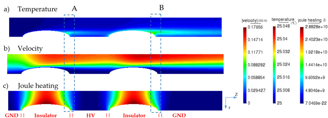
Figure 5. Simulation results for the liquid's (a) temperature, (b) velocity, and (c) joule heating along the z-axis at the first treatment chamber ( N_{HV1} ).
