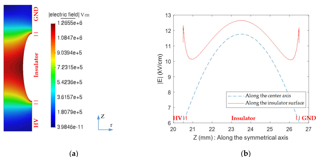
Figure 4. Simulation results for (a) Electric field intensity, and (b) electric field intensity distribution along the insulator surface and symmetrical line in the first treatment zone.
