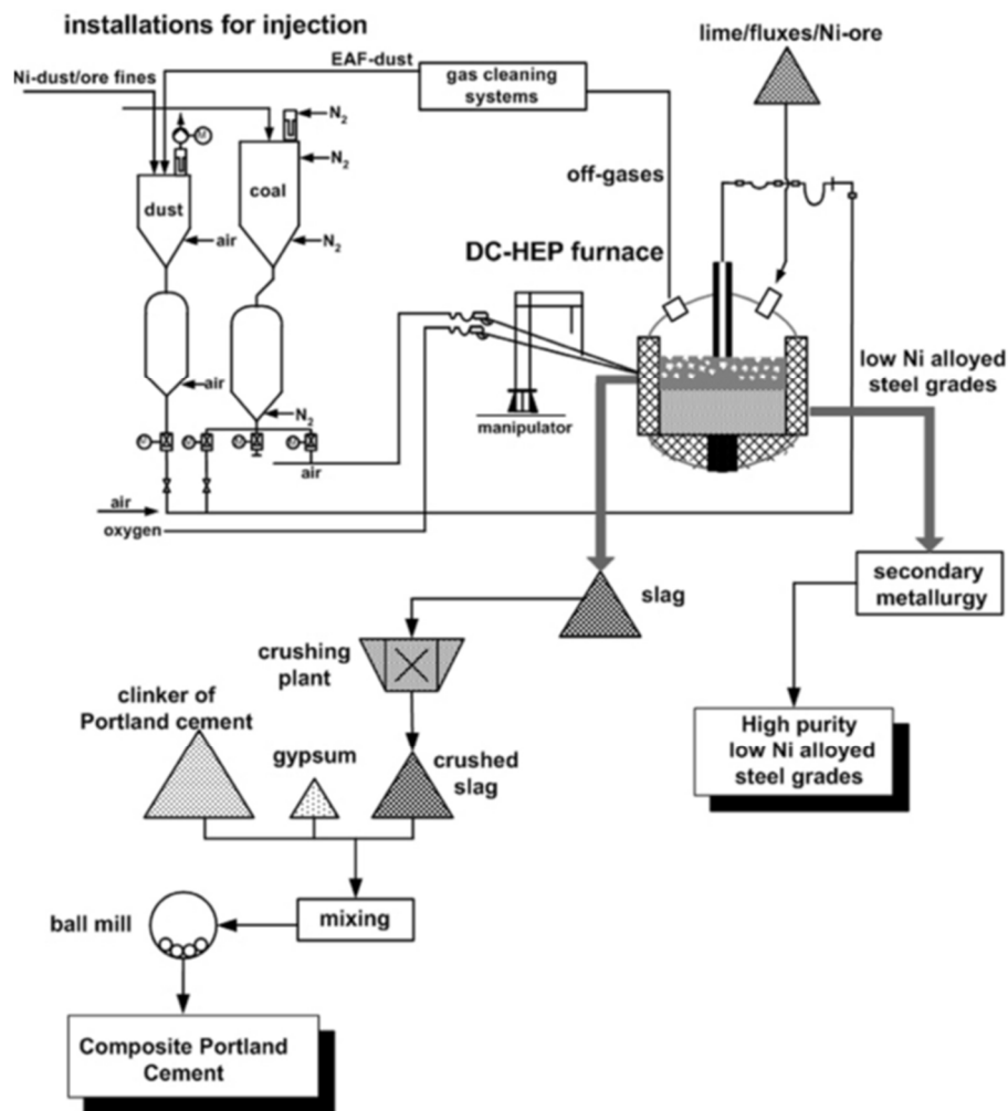
Figure S1. Flow sheet of the zero residues production smelting process for metallurgical dusts and ore fines recycling [1].
