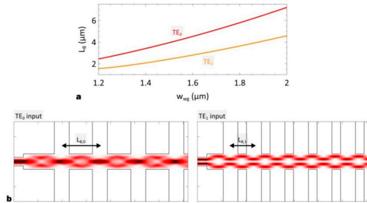
Figure 14. (a) The calculated beat lengths ( L_B ) for TE 0 and TE 1 modes with varied waveguide width ( w_{wg} ). (b) The calculated light propagation profiles for MMI-based crossings when TE 0 (left panel) and TE 1 (right panel) are launched. The beat lengths are different between TE 0 and TE 1 .
