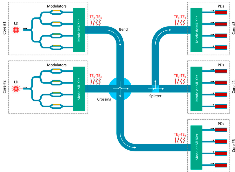
Figure 11. The configuration for MDM-enabled interconnects with multi-mode routing devices.
