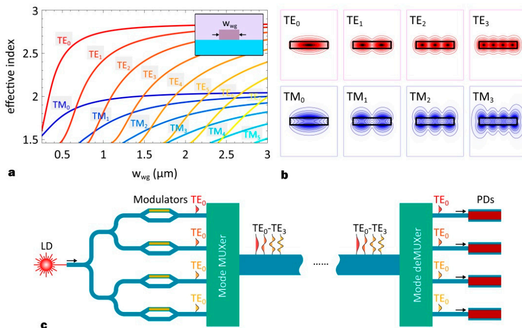
Figure 1. (a) The calculated effective indices for the higher-order modes in a silicon-on-insulator (SOI) waveguide with varied waveguide width ( w_{\text{wg}} ). The inset shows the cross-section of a multi-mode SOI waveguide with some key parameters labeled. (b) The calculated field profiles for the first four transverse electric (TE) and transverse magnetic (TM) modes. (c) The configuration for a typical four-channel mode-division multiplexing (MDM) system.
