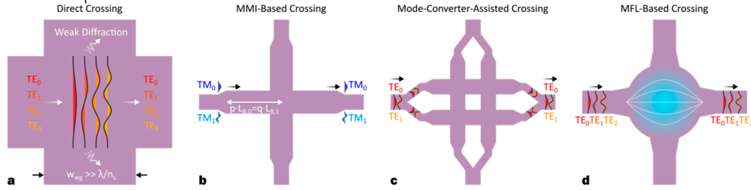
Figure 15. The schematics for different silicon multi-mode crossings: (a) direct crossing [194], (b) MMI-based crossing [197,198], (c) mode converter-assisted crossing [199,200], (d) Maxwell's fisheye lens (MFL)-based crossing [201,202].
