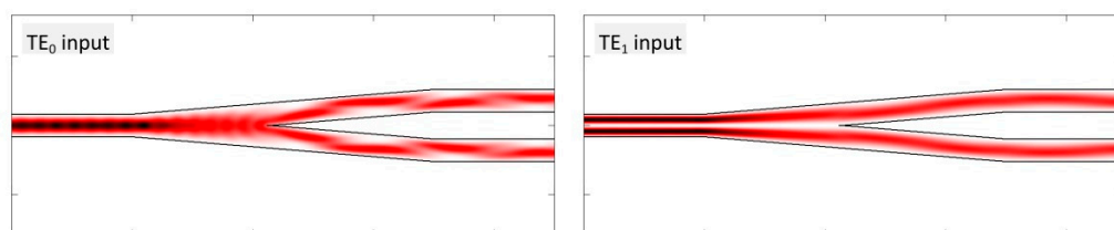
Figure 16. The calculated light propagation profiles for a Y-junction when TE_0 (left panel) and TE_1 (right panel) are launched. The mode order cannot be preserved in the splitting process.
