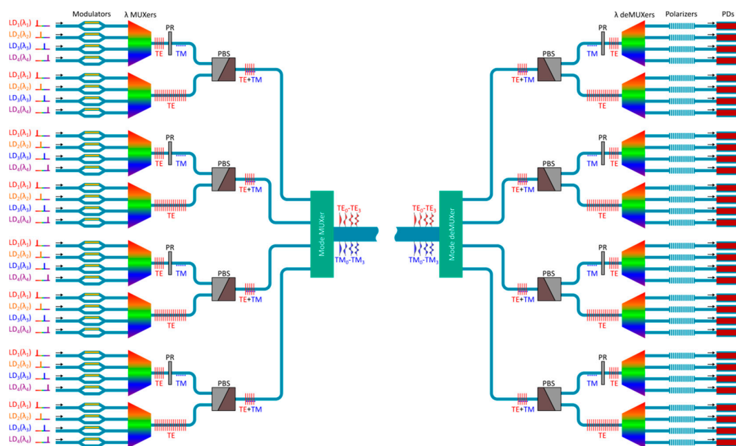
Figure 9. A proposal for the scalable WDM/polarization-division multiplexing (PDM)/MDM hybrid systems.
