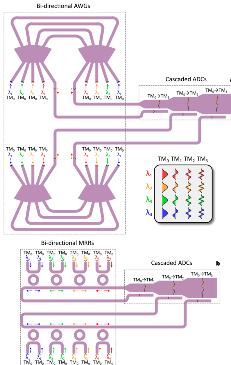
Figure 6. The schematics for the silicon wavelength/mode hybrid (de)multiplexers with (a) bi-directional arrayed waveguide gratings (AWGs) [92] and (b) bi-directional micro-ring resonators (MRRs) [94]. The inset shows the wavelength and mode channel arrangement. Here, a 4 \times 4 wavelength-division multiplexing (WDM)/MDM system is illustrated as an example.
