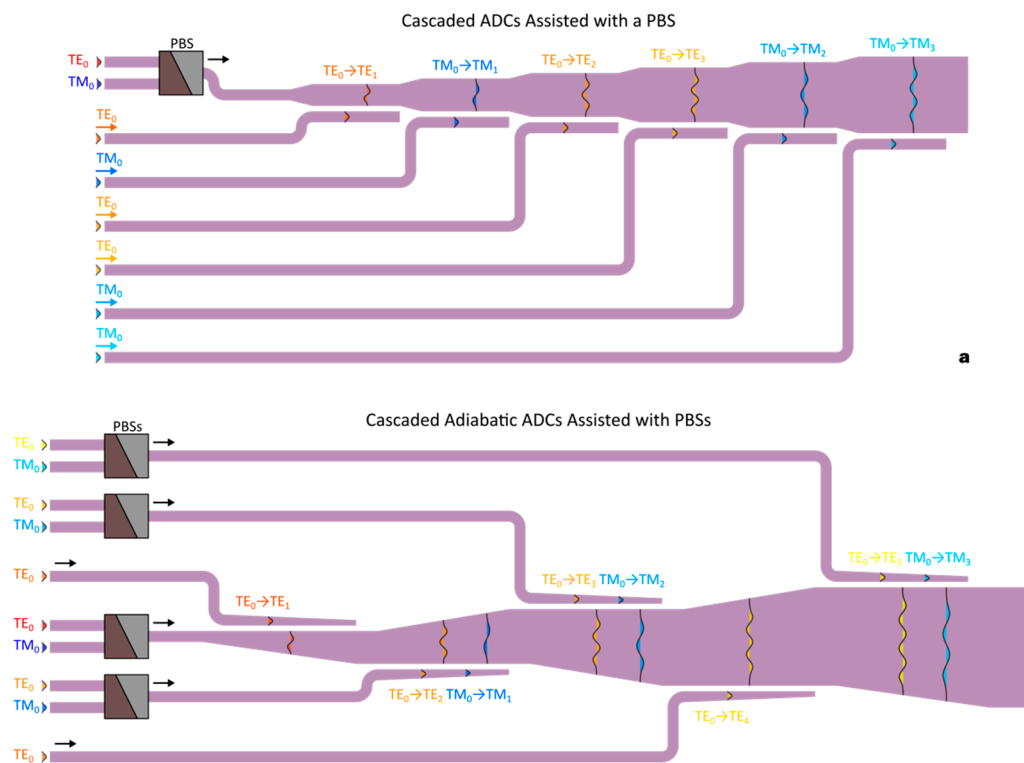
Figure 7. The schematics for the silicon polarization/mode hybrid (de)multiplexers based on (a) cascaded ADCs [96] and (b) cascaded adiabatic ADCs [100].
