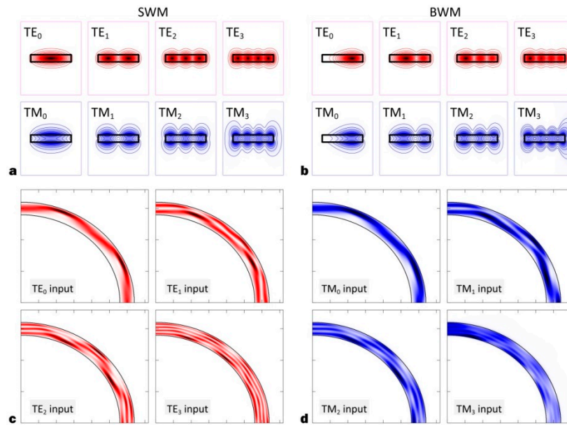
Figure 12. The calculated field profiles for (a) straight-waveguide mode (SWM) and (b) bent-waveguide mode (BWM). The calculated light propagation profiles for a 15-μm multi-mode bend when (c) TE 0-3 and (d) TM 0-3 modes are launched.
