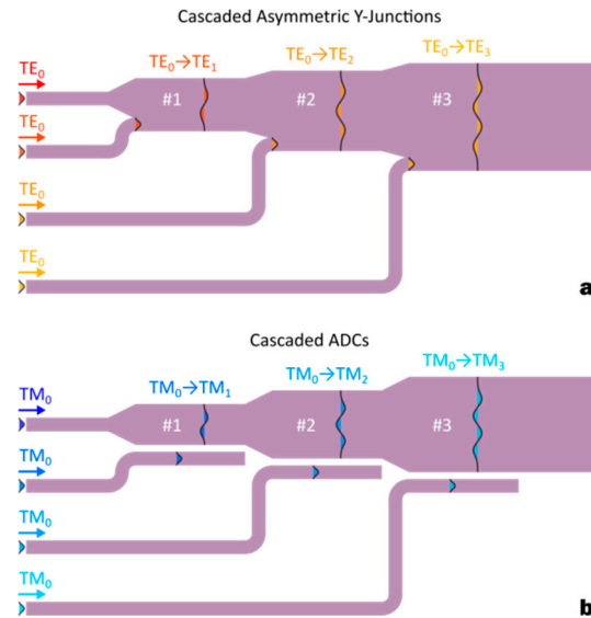
Figure 5. The schematics for the scalable silicon mode (de)multiplexers based on (a) cascaded asymmetric Y-junctions [75,76] and (b) cascaded ADCs [77].
