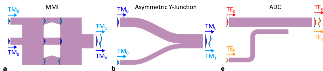
Figure 3. The schematics for the silicon few-mode (de)multiplexers based on (a) multimode interference couplers (MMI) [24], (b) asymmetric Y-junction [29] and (c) asymmetric directional coupler (ADC) [36].
