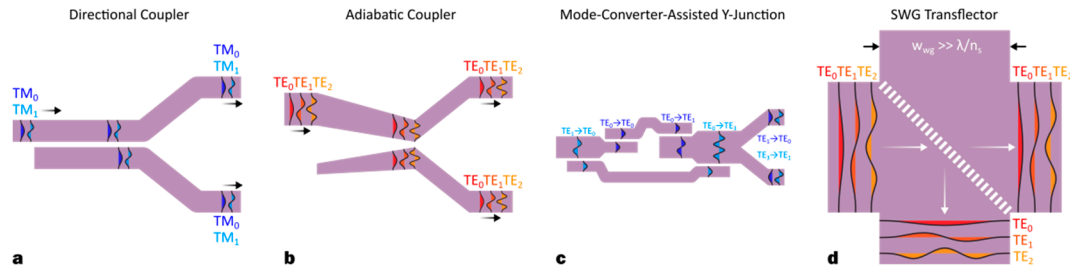
Figure 17. The schematics for different silicon multi-mode splitters based on (a) directional coupler [211], (b) adiabatic coupler [212], (c) mode converter-assisted Y-junction [213], (d) subwavelength grating (SWG) transfecter [214].
