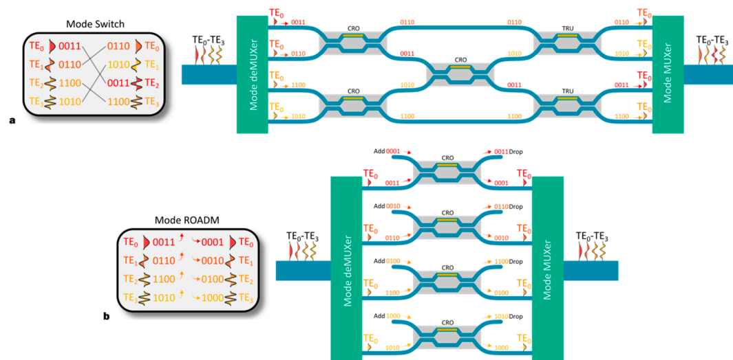
Figure 19. The configurations for (a) mode switch [245] and (b) mode reconfigurable optical add-drop multiplexers (ROADM) [250]. The insets show the mapping relation between signals and modes. Here, a four-channel MDM system is illustrated as an example.
