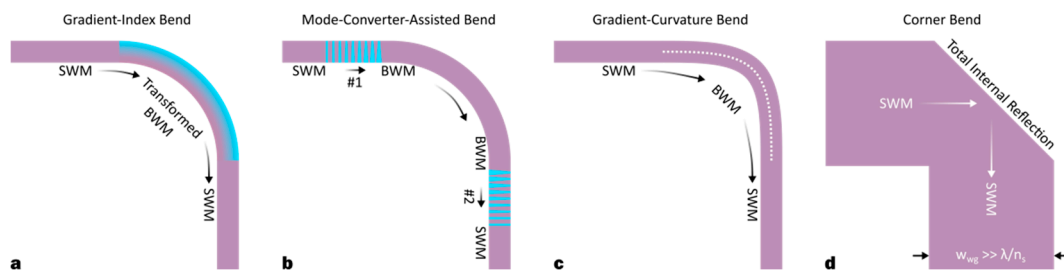
Figure 13. The schematics for different silicon multi-mode bends: (a) gradient index bend [167,168], (b) mode converter-assisted bend [170], (c) gradient curvature bend [171], (d) corner bend [172].
