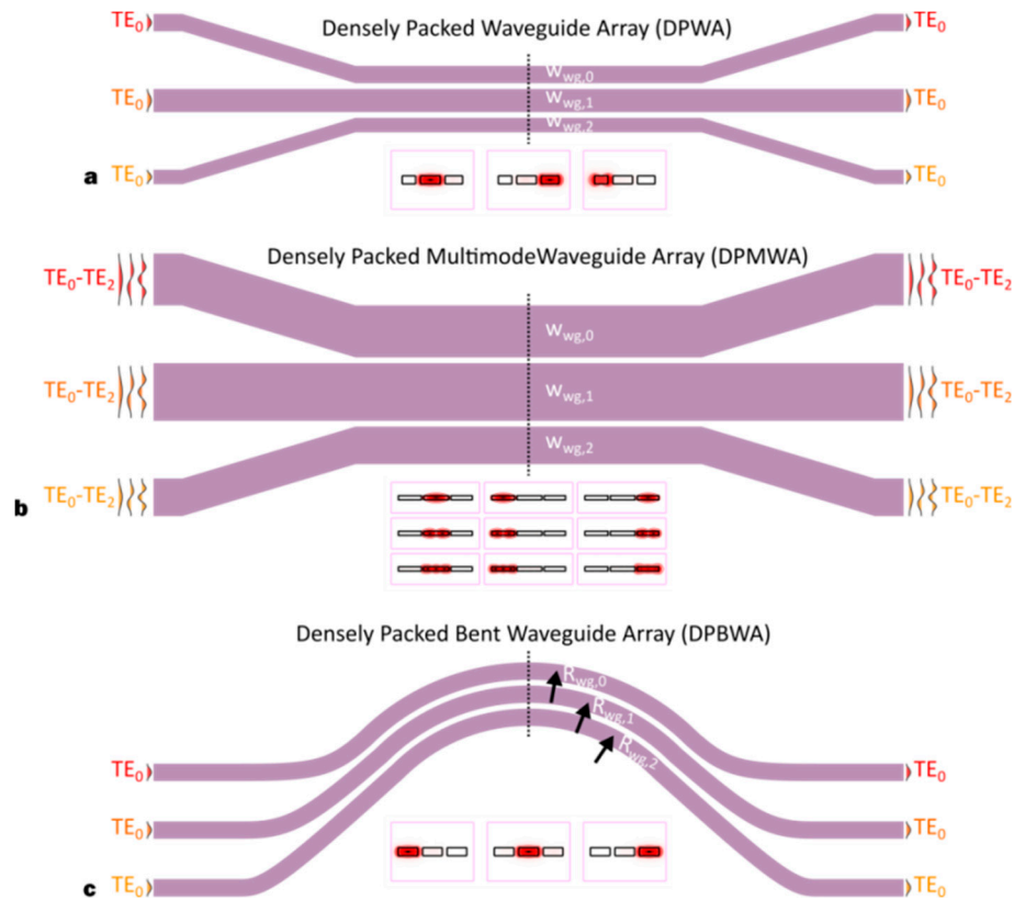
Figure 10. The schematics for the silicon (a) densely packed waveguide array (DPWA) [154,157], (b) densely packed multi-mode waveguide array (DPMWA) [158] and (c) densely packed bent-waveguide array (DPBWA) [159,160].
