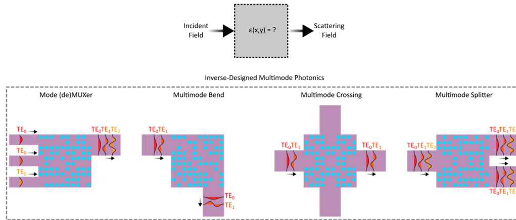
Figure 18. Upper panel: the schematic for photonic inverse-design. Lower panel: the schematic for inverse-designed mode (de)multiplexer [85], multi-mode bend [175], multi-mode crossing [204] and multi-mode splitter [220].
