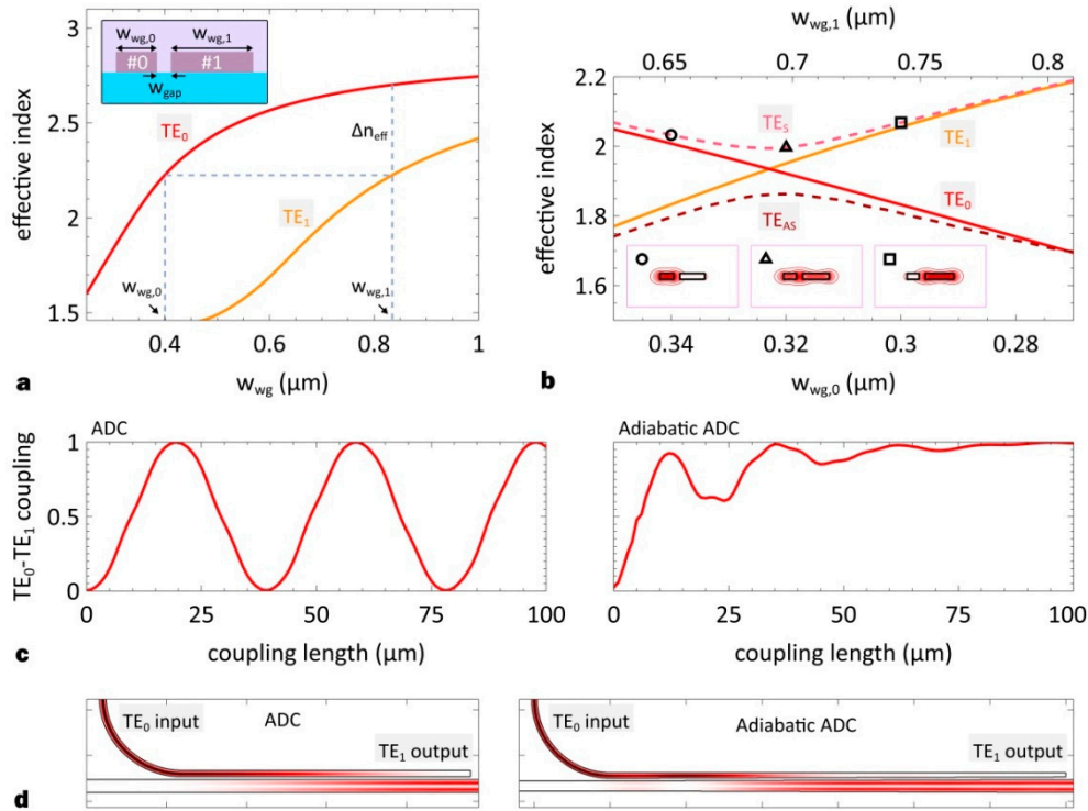
Figure 4. (a) The calculated effective indices for TE 0 and TE 1 modes in a SOI waveguide with varied waveguide width ( w_{wg} ). The inset shows the cross-section of an ADC with some key parameters labeled. (b) The calculated effective indices for TE 0 and TE 1 modes (solid lines) and TE s /TE AS super-modes (dashed lines) in an ADC with varied waveguide width ( w_{wg,0} and w_{wg,1} ). The inset shows the mode profiles. (c) The calculated TE 0 -TE 1 coupling ratio for ADC (left panel) and adiabatic ADC (right panel) with varied coupling length. (d) The calculated light propagation profiles for ADC (left panel) and adiabatic ADC (right panel) when TE 0 mode is launched.
