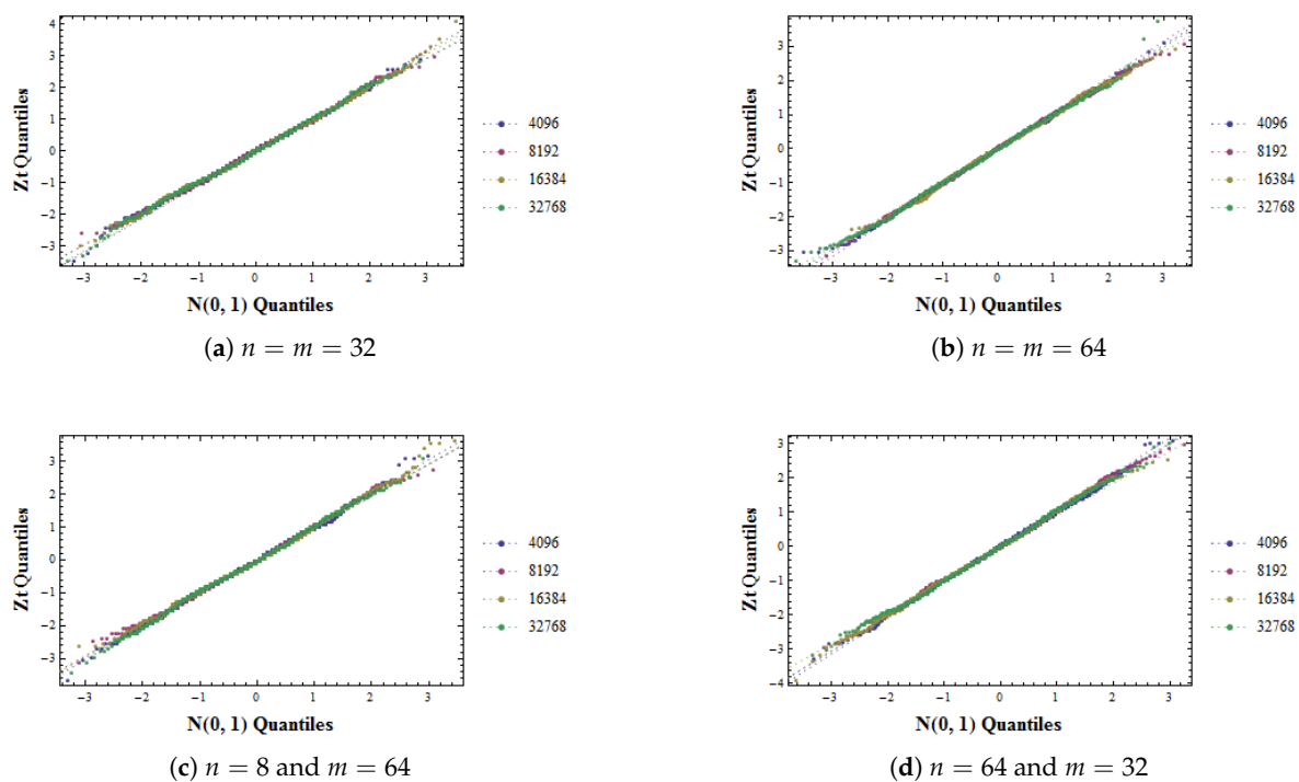
Figure 2. Adjustment of the observed distribution from Z_T to N(0, 1) in H^i random matrices, which satisfy the BIC.
