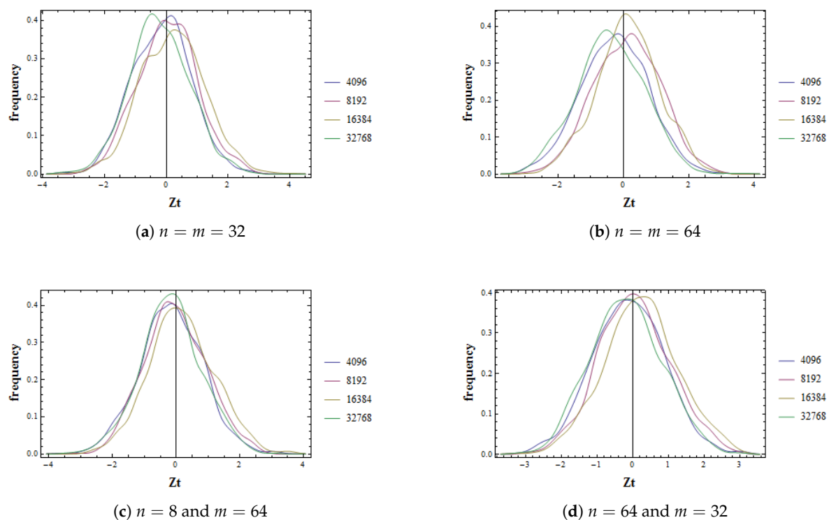
Figure 1. Observed distribution of 1000 values of Z_T in random H^i matrices for various values of n , m , and l .
