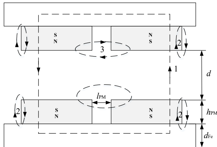
Figure 9. 2D model of the coreless double-sided AFPMSM with dimensions.
