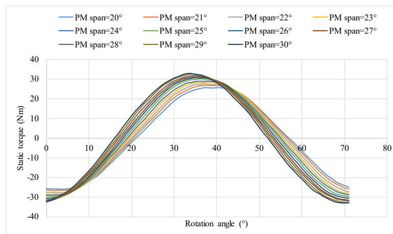
Figure 6. PM span influence on the torque size of the machine.
