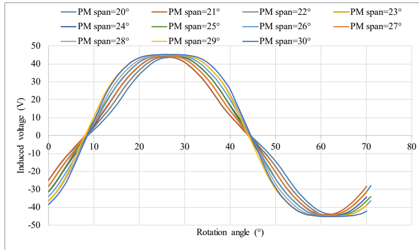
Figure 7. PM span influence on the induced voltage size of the machine.
