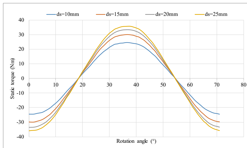
Figure 8. Stator thickness influence on the torque size of the machine.
