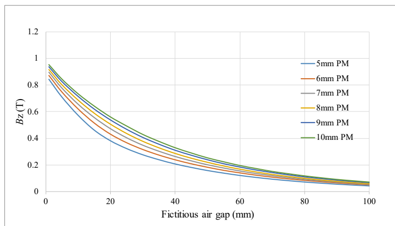
Figure 4. Influence of PM thickness on the size of B_z .
