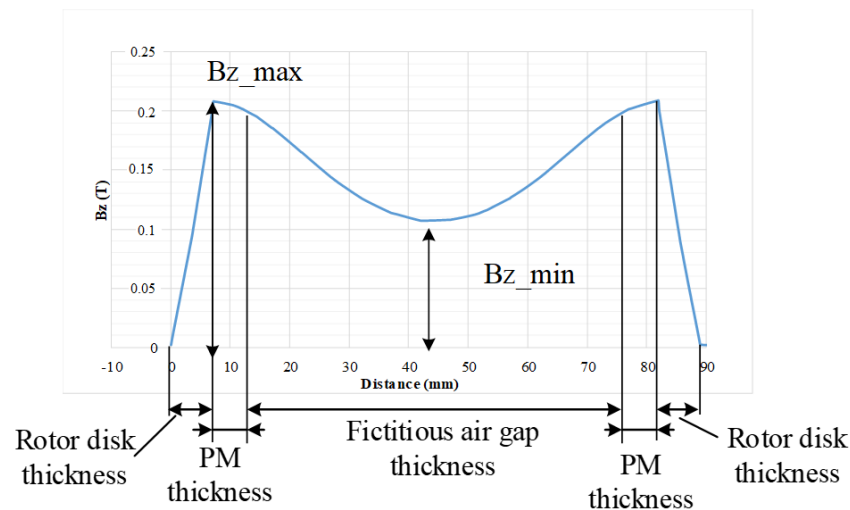
Figure 2. Axial component of magnetic flux density along the centerline (an example is shown at 55-mm virtual air gap thickness, 7-mm rotor disk thickness and 5-mm PM thickness. Values of B_z near the PM ( B_{z\_max} ) and at the middle of the virtual air gap ( B_{z\_min} ) are shown).
