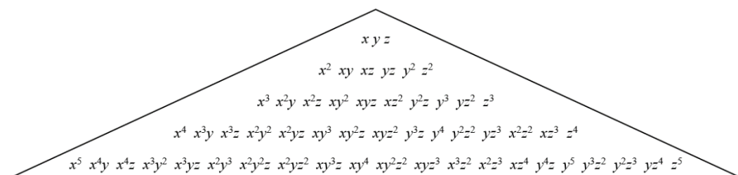
Figure 3. Pascal triangle for function with three unknowns.
