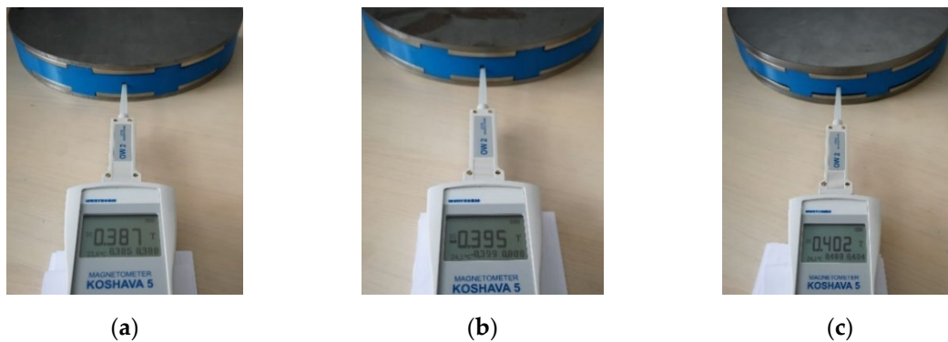
Figure 11. Measuring procedure for with the developed tool ( d = 22 mm) with 5-mm PM thickness and different rotor disk thicknesses: h_{TM} = 5 mm: (a) d_{Fe} = 5 mm, (b) d_{Fe} = 6 mm, (c) d_{Fe} = 10 mm.
