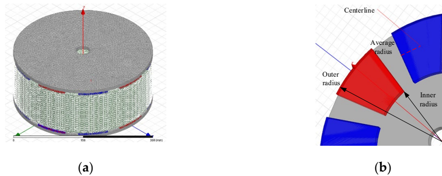
Figure 1. Simplified finite element method (FEM) model: (a) 3D model of the simplified axial flux permanent magnet synchronous machine (AFPMSM), and (b) model of rotor disk with surface-mounted permanent magnets (PMs) with their dimensions and the position of the centerline on which the axial component of magnetic flux density is analyzed.
