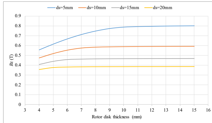
Figure 5. Rotor disks thickness influence on the size of B_z .
