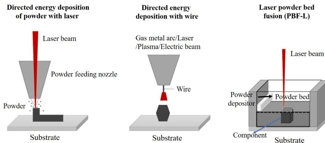
Figure 4. Schematics of main additive manufacturing processes.
