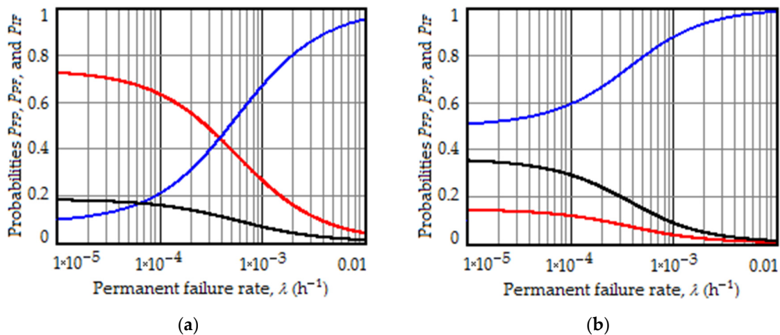
Figure 8. Dependences of the posterior probabilities of dismounting the LRU due to the in-flight false-positive (red curve), intermittent fault (black curve), and permanent failure (blue curve) on the permanent failure rate when \theta = 10^{-4} \text{ h}^{-1} ; (a) P_{flight}^{FP} = 1 \times 10^{-3} ; (b) P_{flight}^{FP} = 1 \times 10^{-4} .
