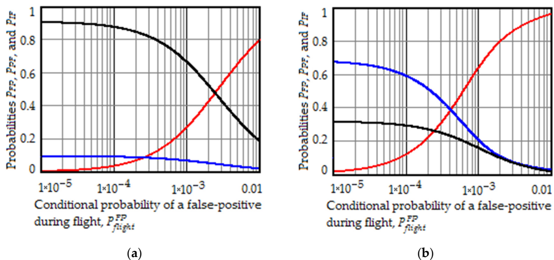
Figure 6. Dependences of the posterior probabilities of dismantling the LRU due to the in-flight false-positive (red curve), intermittent fault (black curve), and permanent failure (blue curve) on the conditional probability of in-flight false-positive when \lambda = 10^{-4} h -1 ; (a) \theta = 1 \times 10^{-3} h -1 ; (b) \theta = 1 \times 10^{-4} h -1 .
