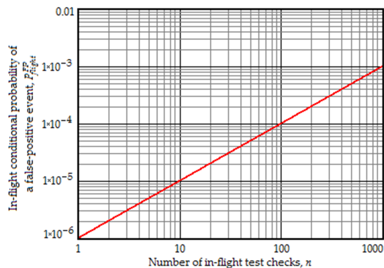
Figure 2. The dependency of the in-flight conditional probability of a false-positive event on the number of test checks.
