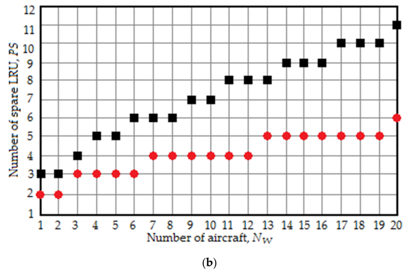
Figure 4. The dependency of the optimal quantity of spare LRU versus the quantity of aircraft for the first WM option; (a) Red circles: P_{flight}^{FP} = 1 \times 10^{-4} , black squares: P_{flight}^{FP} = 1 \times 10^{-3} ; (b) Red circles: \theta = 1 \times 10^{-4} \text{ h}^{-1} , black squares: \theta = 1 \times 10^{-3} \text{ h}^{-1} .
