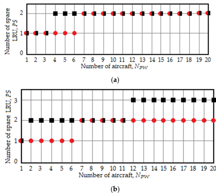
Figure 14. The dependency of the optimal number of spare LRU on the number of aircraft for the fourth and fifth PWM options; (a) \theta = 1 \times 10^{-4} \text{ h}^{-1} , red circles: P_{flight}^{FP} = 1 \times 10^{-4} , black squares: P_{flight}^{FP} = 1 \times 10^{-3} ; (b) P_{flight}^{FP} = 1 \times 10^{-4} , red circles: \theta = 1 \times 10^{-4} \text{ h}^{-1} , black squares: \theta = 1 \times 10^{-3} \text{ h}^{-1} .
