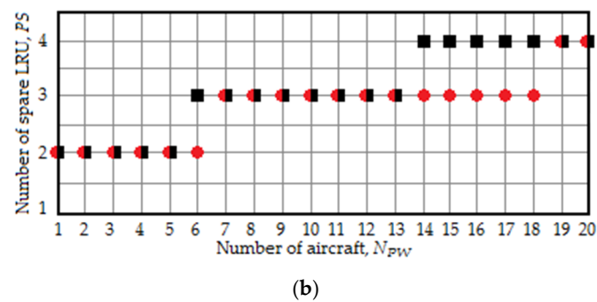
Figure 12. The dependency of the optimal quantity of spare LRU on the quantity of aircraft for the second PWM option; (a) \theta = 1 \times 10^{-4} \text{ h}^{-1} , red circles: P_{flight}^{FP} = 1 \times 10^{-4} , black squares: P_{flight}^{FP} = 1 \times 10^{-3} ; (b) P_{flight}^{FP} = 1 \times 10^{-4} , red circles: \theta = 1 \times 10^{-4} \text{ h}^{-1} , black squares: \theta = 1 \times 10^{-3} \text{ h}^{-1} .
