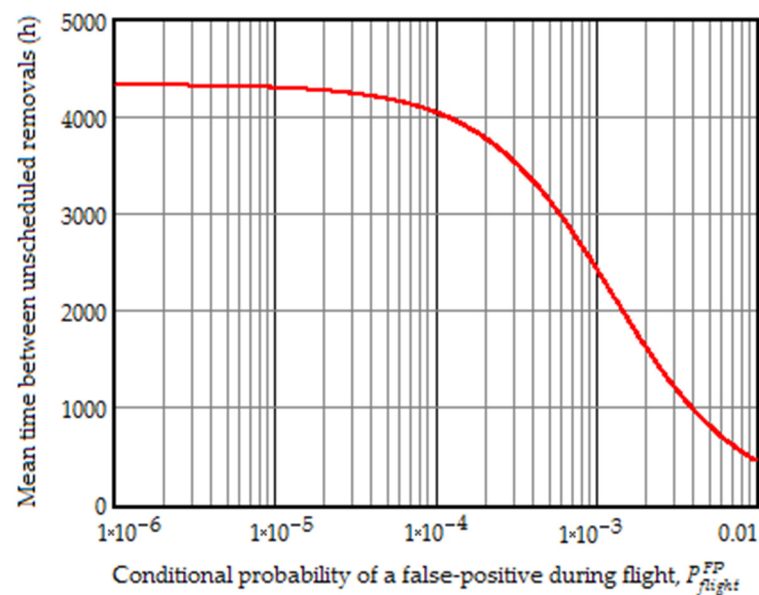
Figure 1. The dependency of MTBUR on the conditional probability of false-positive during flight.
