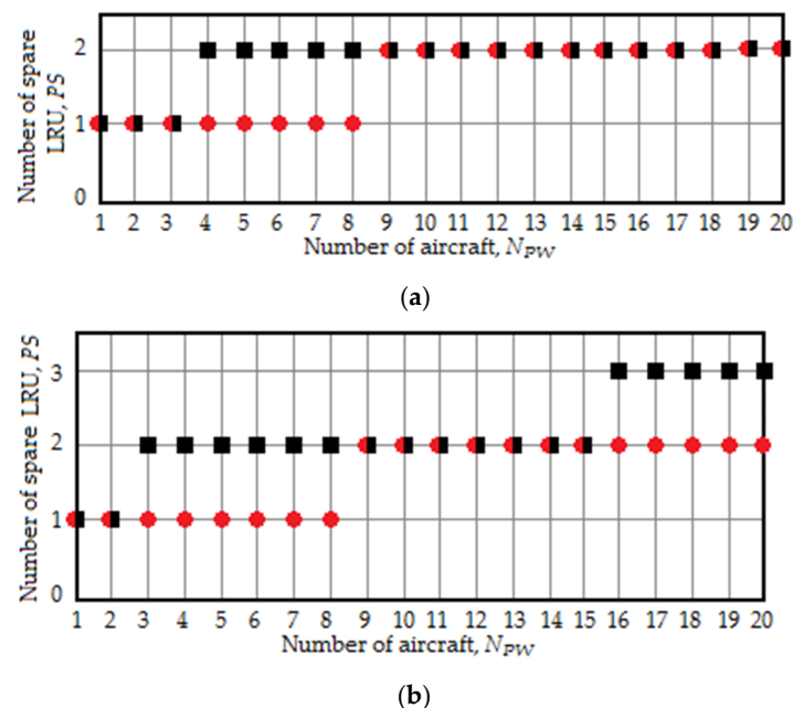
Figure 13. The dependency of the optimal quantity of spare LRU on the quantity of aircraft for the third PWM option; (a) \theta = 1 \times 10^{-4} \text{ h}^{-1} , red circles: P_{flight}^{FP} = 1 \times 10^{-4} , black squares: P_{flight}^{FP} = 1 \times 10^{-3} ; (b) P_{flight}^{FP} = 1 \times 10^{-4} , red circles: \theta = 1 \times 10^{-4} \text{ h}^{-1} , black squares: \theta = 1 \times 10^{-3} \text{ h}^{-1} .
