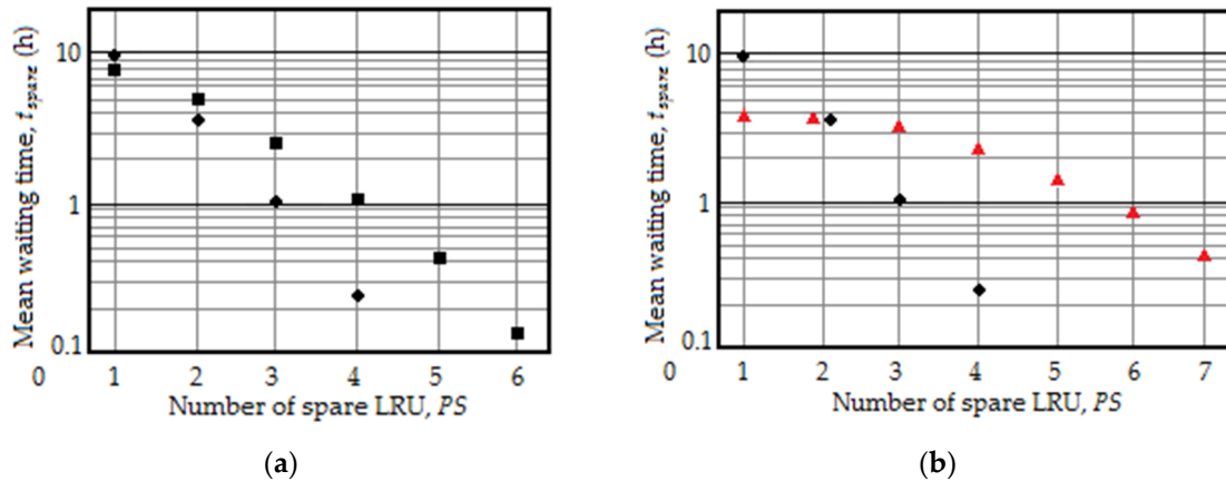
Figure 3. Dependences of the mean waiting time on the number of planned spare LRU ( PS ) for the first WM option; (a) circles: P_{flight}^{FP} = 1 \times 10^{-4} , squares: P_{flight}^{FP} = 1 \times 10^{-3} ; (b) black circles: \theta = 1 \times 10^{-4} \text{ h}^{-1} , red triangles: \theta = 1 \times 10^{-3} \text{ h}^{-1} .
