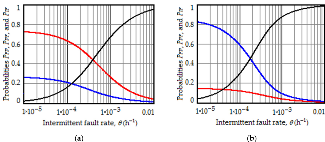
Figure 7. Dependences of the posterior probabilities of dismantling the LRU due to the in-flight false-positive (red curve), intermittent fault (black curve), and permanent failure (blue curve) on the intermittent fault rate when \lambda = 10^{-4} h -1 ; (a) P_{flight}^{FP} = 1 \times 10^{-3} ; (b) P_{flight}^{FP} = 1 \times 10^{-4} .
