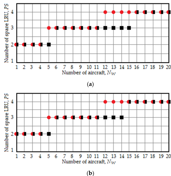
Figure 10. The dependency of the optimal quantity of spare LRU on the quantity of aircraft for the second WM option; (a) Red circles: P_{flight}^{FP} = 1 \times 10^{-4} , black squares: P_{flight}^{FP} = 1 \times 10^{-3} ; (b) Red circles: \theta = 1 \times 10^{-4} \text{ h}^{-1} , black squares: \theta = 1 \times 10^{-3} \text{ h}^{-1} .
