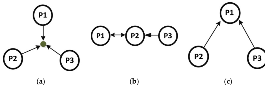
Figure 15. Selection of formation reference points: (a) Take the green dot, in the center of P1 P2 P3, as a reference. (b) P1 and P3 take neighbor P2 as a reference, P2 takes the nearest neighbor P1 as a reference. (c) Take the leading robot P1 of P2 and P3 as a reference.
