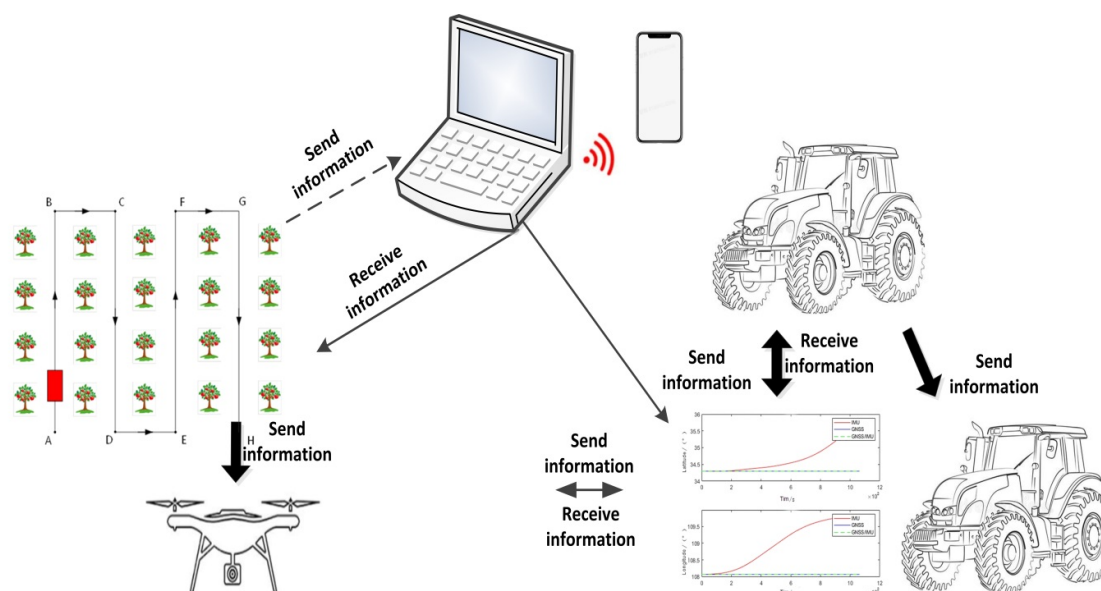
Figure 18. The computer as the center controller was used to send initial paths for UGVs and UAVs control units through communication. And perception data were exchanged between multi-robots and computers.UGV.
