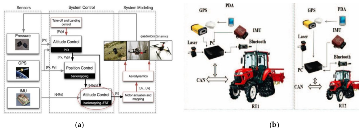
Figure 6. Heterogeneous sensors carried by agricultural multi-robots. (a) Typical sensors for aerial robots: inertial measurement unit (IMU), Global Positioning System (GPS), and pressure gauge [28]. (b) Typical sensor for ground robots RT1 and RT2: GPS, Laser, and IMU [45].
