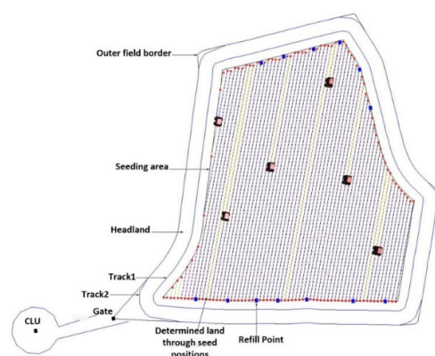
Figure 9. A centralized entity was used to plan the seeding task, seeding patterns, and seed densities for different robots in the simulation environment. At the same time, the centralized entities were used to monitor the whole seeding process to avoid collisions between robots [58]. The small blue dots are the locations of the seeds planned to be sown, the yellow dots are the seeds that have been successfully planted, and the larger red dots are the border seed sowing locations.
