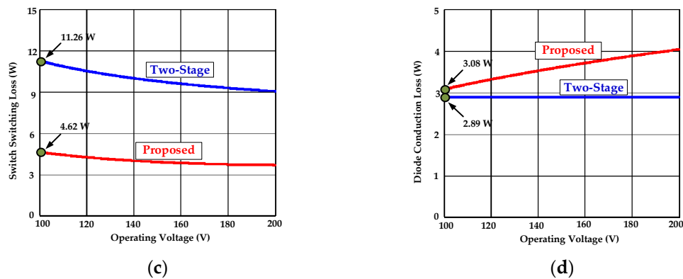
Figure 9. The power loss comparison curves of the proposed inverter and the traditional two-stage system: (a) conduction loss of all inductors; (b) conduction loss of all switches; (c) switching loss of all switches; (d) conduction loss of all diodes.
