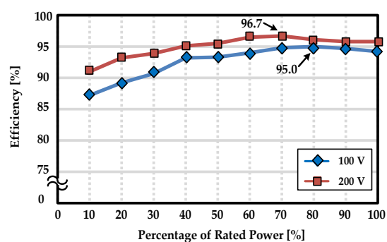
Figure 18. Measured efficiency curves of the laboratory prototype.
