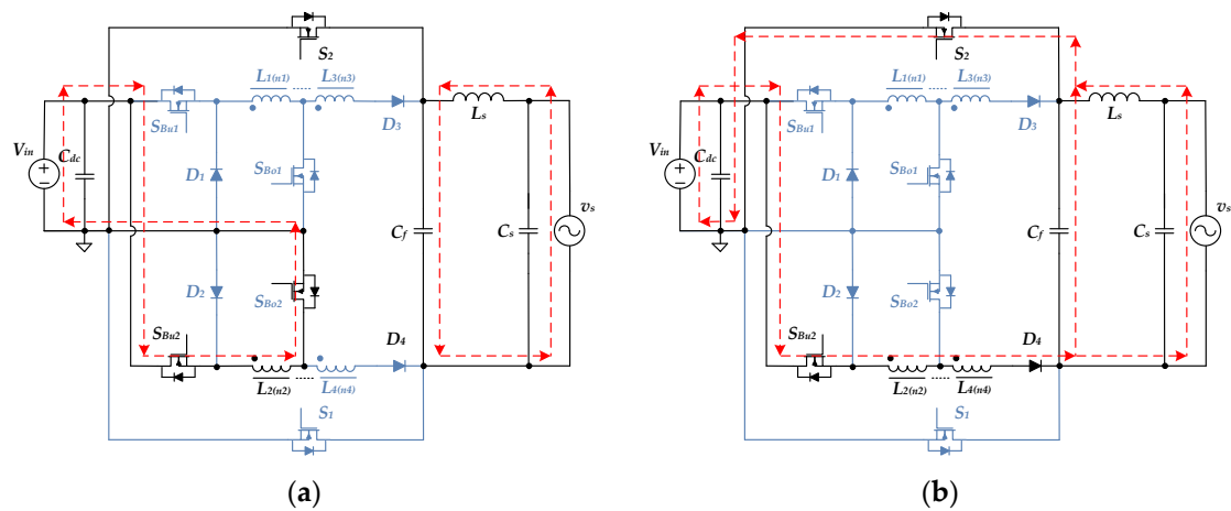
Figure 8. During the negative half-cycle, the corresponding circuits of step-up mode: (a) S_{Bu1} OFF, S_{Bu2} ON, S_{Bo1} OFF, S_{Bo2} ON, S_1 OFF, and S_2 ON; (b) S_{Bu1} OFF, S_{Bu2} ON, S_{Bo1} OFF, S_{Bo2} OFF, S_1 OFF, and S_2 ON.
