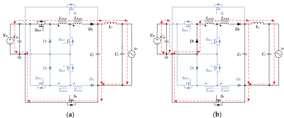
Figure 5. During the positive half-cycle, the corresponding circuits of step-down mode: (a) S_{Bu1} ON, S_{Bu2} OFF, S_{Bo1} OFF, S_{Bo2} OFF, S_1 ON, and S_2 OFF; (b) S_{Bu1} OFF, S_{Bu2} OFF, S_{Bo1} OFF, S_{Bo2} OFF, S_1 ON, and S_2 OFF.
