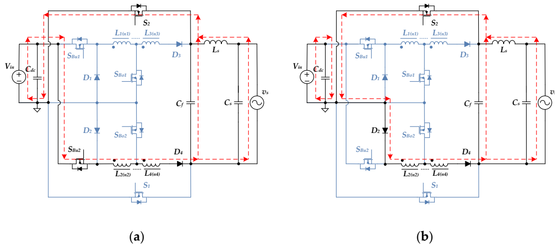
Figure 6. During the negative half-cycle, the corresponding circuits of step-down mode: (a) S_{Bu1} OFF, S_{Bu2} ON, S_{Bo1} OFF, S_{Bo2} OFF, S_1 OFF, and S_2 ON; (b) S_{Bu1} OFF, S_{Bu2} OFF, S_{Bo1} OFF, S_{Bo2} OFF, S_1 OFF, and S_2 ON.
