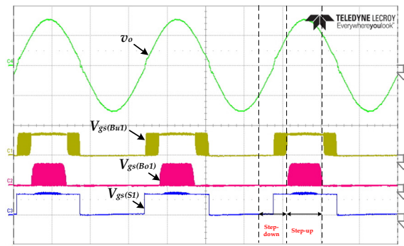
Figure 14. The experimental waveforms of the output voltage v_o and the gate-driving signals under the condition of 200 V input voltage and 500 W load ( v_o : 200 V/div; V_{GS} : 20 V/div; time: 5 ms/div).
