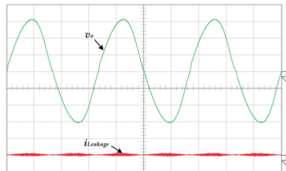
Figure 13. The simulation waveforms of the output voltage v_o and the leakage current i_{Leakage} under the condition of 100 V input voltage and 500 W load ( v_o : 100 V/div; i_{Leakage} : 100 mA/div; time: 5 ms/div).
