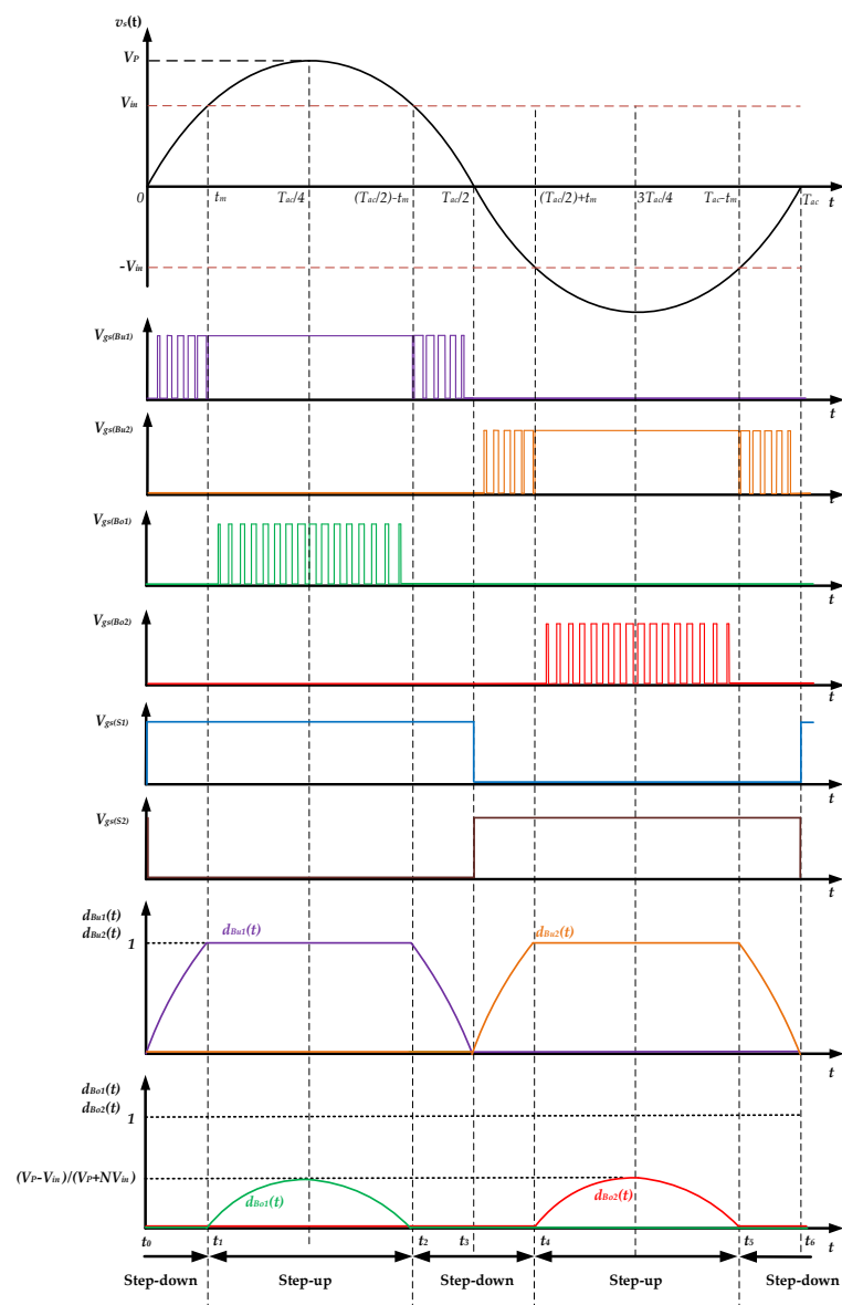
Figure 4. The timing diagram of working modes and switch driving signals.
