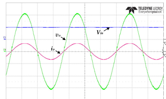
Figure 11. The experimental waveforms of the input voltage V_{in} , the output voltage v_o , and the output current i_o under the condition of 100 V input voltage and 500 W load ( V_{in} , v_o : 100 V/div; i_o : 5 A/div; time: 5 ms/div).
