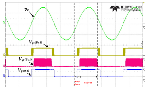
Figure 10. The experimental waveforms of the output voltage v_o and the gate-driving signals under the condition of 100 V input voltage and 500 W load. ( v_o : 200 V/div; V_{gs} : 20 V/div; time: 5 ms/div).
