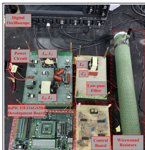
Figure 19. The picture with the experimental test bench.
