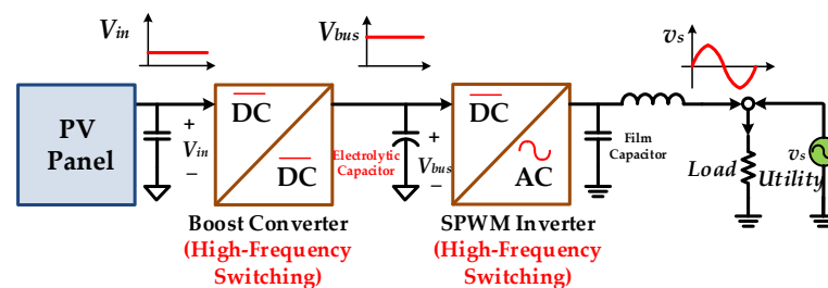
Figure 1. The PV grid-tied system with two stage of energy processing.
