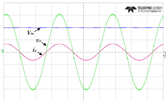
Figure 15. The experimental waveforms of the input voltage V_{in} , the output voltage v_o , and the output current i_o under the condition of 200 V input voltage and 500 W load ( V_{in} , v_o : 100 V/div; i_o : 5 A/div; time: 5 ms/div).
