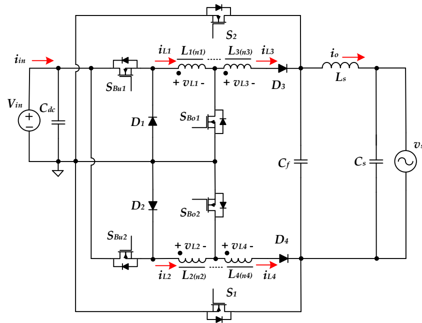
Figure 3. The schematic of the investigated transformer-less buck-boost grid-tied inverter.
