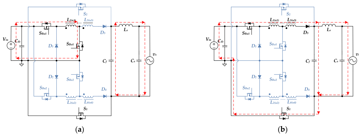
Figure 7. During the positive half-cycle, the corresponding circuits of step-up mode: (a) S_{Bu1} ON, S_{Bu2} OFF, S_{Bo1} ON, S_{Bo2} OFF, S_1 ON, and S_2 OFF; (b) S_{Bu1} ON, S_{Bu2} OFF, S_{Bo1} OFF, S_{Bo2} OFF, S_1 ON, and S_2 OFF.
