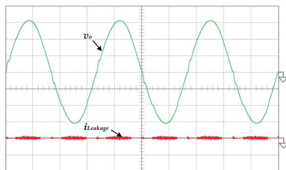
Figure 17. The simulation waveforms of the output voltage v_o and the leakage current i_{Leakage} under the condition of 200 V input voltage and 500 W load ( v_o : 100 V/div; i_{Leakage} : 100 mA/div; time: 5 ms/div)
