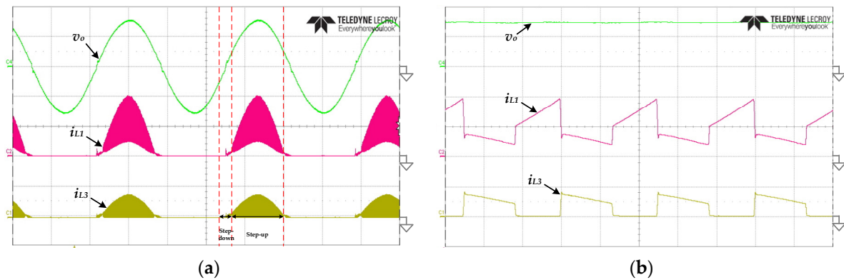
Figure 12. Under the condition of 100 V input voltage and 500 W load, the experimental waveforms of the output voltage v_o and the inductor currents i_{L1} , i_{L3} : (a) complete AC period ( v_o : 200 V/div; i_{L1} , i_{L3} : 10 A/div; time: 5 ms/div); (b) zoom-in on the peak of the output voltage ( v_o : 200 V/div; i_{L1} , i_{L3} : 10 A/div; time: 20 \mu s/div).
