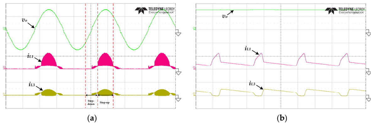
Figure 16. Under the condition of 200 V input voltage and 500 W load, the experimental waveforms of the output voltage v_o and the inductor currents i_{L1} , i_{L3} : (a) complete AC period ( v_o : 200 V/div; i_{L1} , i_{L3} : 10 A/div; time: 5 ms/div); (b) zoom-in near the peak of the output voltage ( v_o : 200 V/div; i_{L1} , i_{L3} : 10 A/div; time: 20 μs/div).
