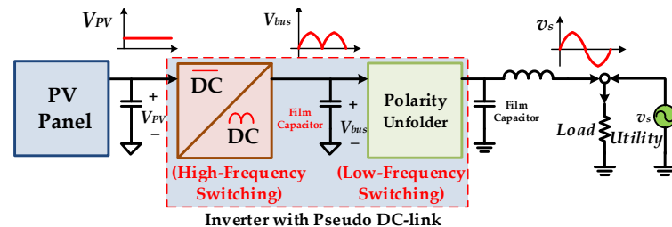
Figure 2. The PV grid-tied system with a single stage of energy processing.
