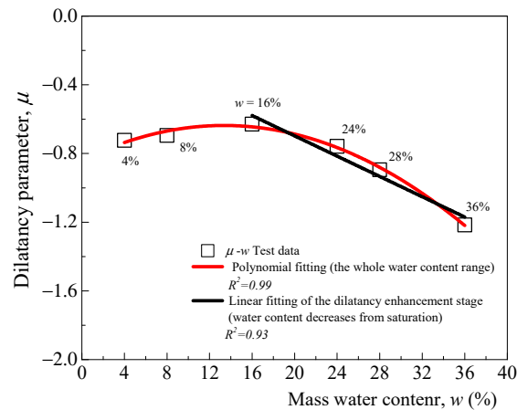
Figure 11. Relationship between the dilatancy parameter \mu and mass water content w .
