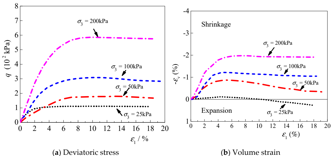
Figure 3. Shear behaviour of the triaxial tests: (a) deviatoric stress; (b) volume strain; (c) stress ratio with the dilatancy rate.
