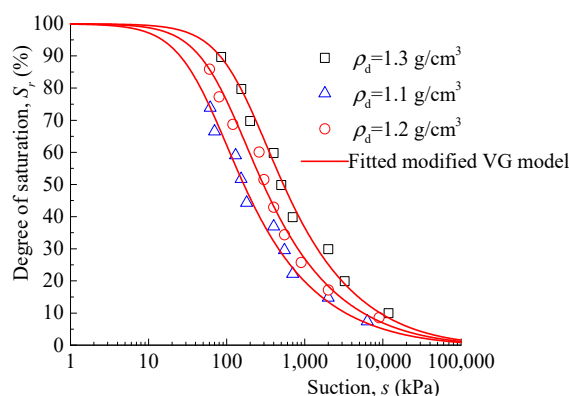
Figure 2. Soil-water characteristic curve.
