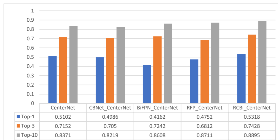
Figure 9. Performance comparison.
