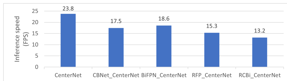
Figure 10. Inference speed.
