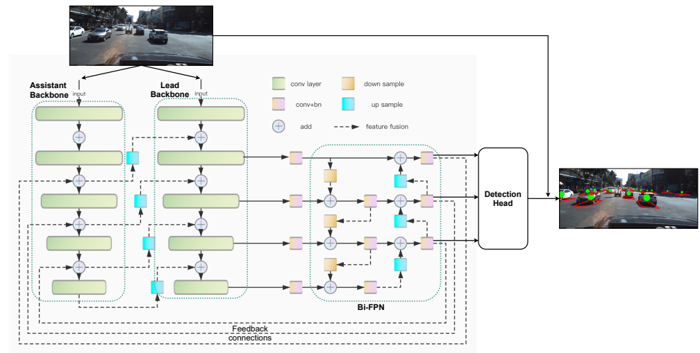
Figure 5. RCBi-CenterNet architecture.
