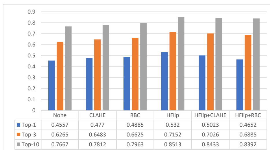
Figure 7. Effects of data augmentation methods.
