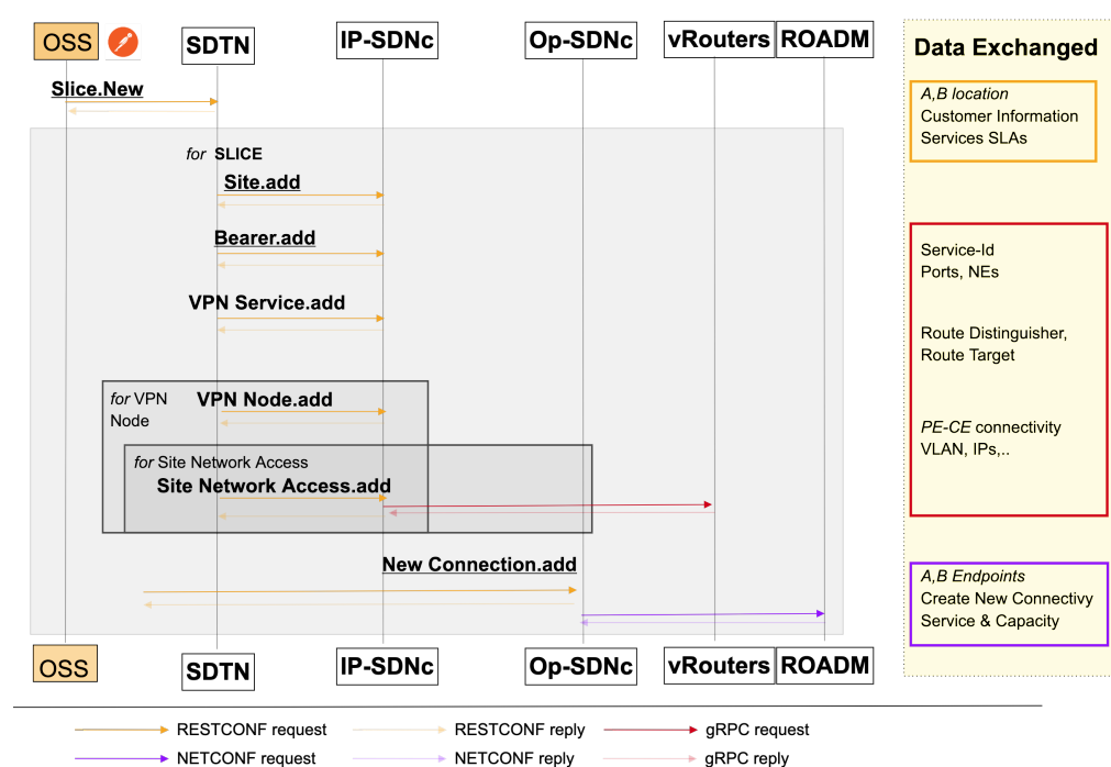
Figure 4. Workflow used to instantiate the network slices in the network. From Postman, a user sends a slice request to the SDTN controller. The SDTN controller automatically split the request based on technological requirements. The L3NM and the T-API are used for the IP and Optical domains, respectively.
