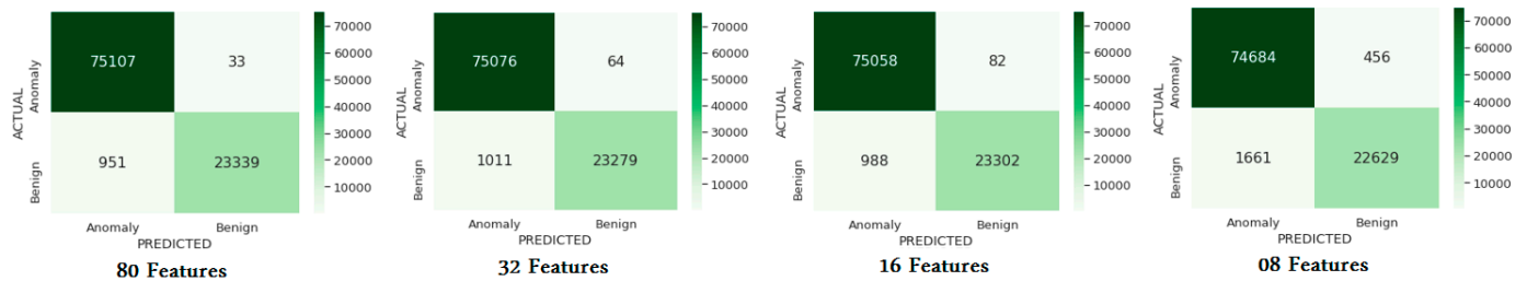
Figure 9. The confusion matrix of DNN-IDS methodology considering the different number of features.
