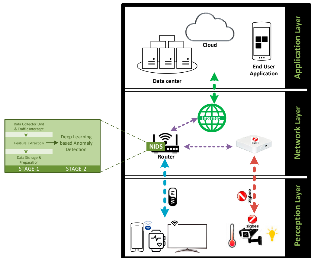
Figure 2. A three-layered IoT architecture.
