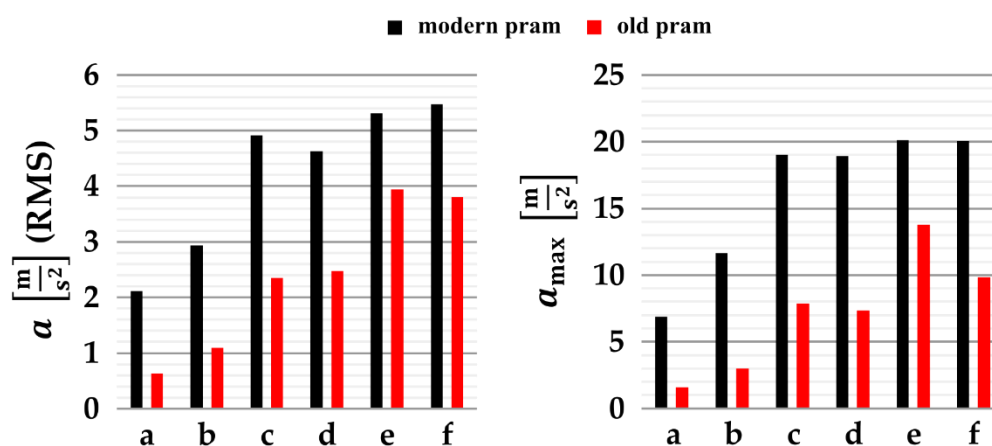
Figure 4. Comparative bar graphs of the RMS and maximum acceleration values from Table 2.
