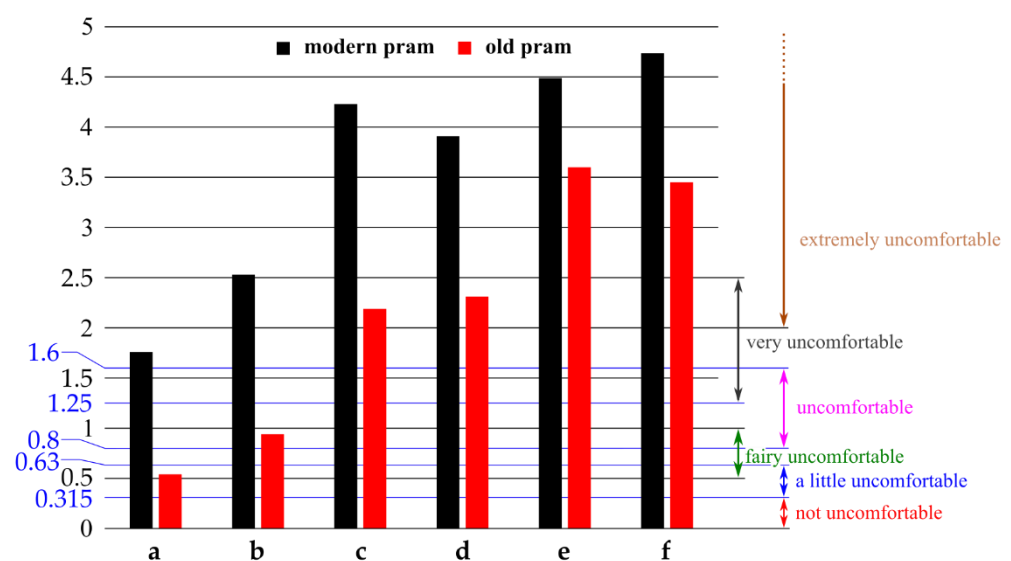
Figure 8. Comparative bar graphs of the weighted RMS acceleration values from ISO 2631-1:1997 [18].
