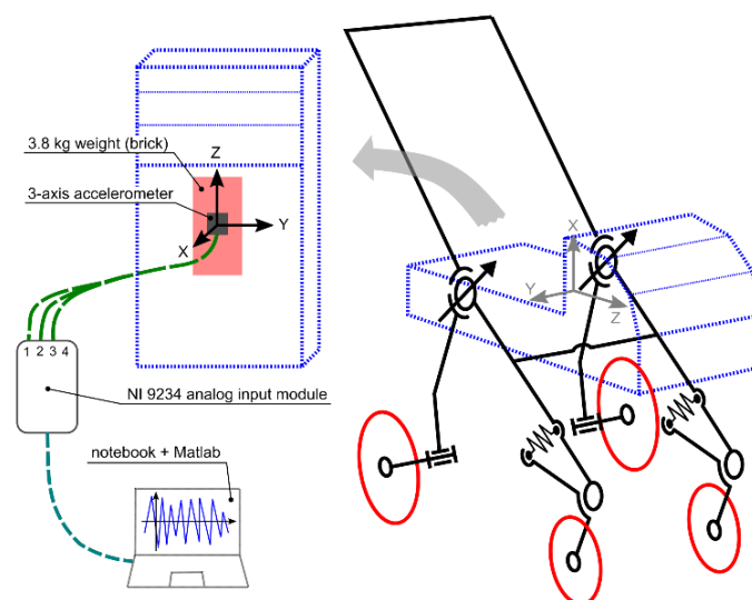
Figure 3. Schematic diagram of the research subject.
