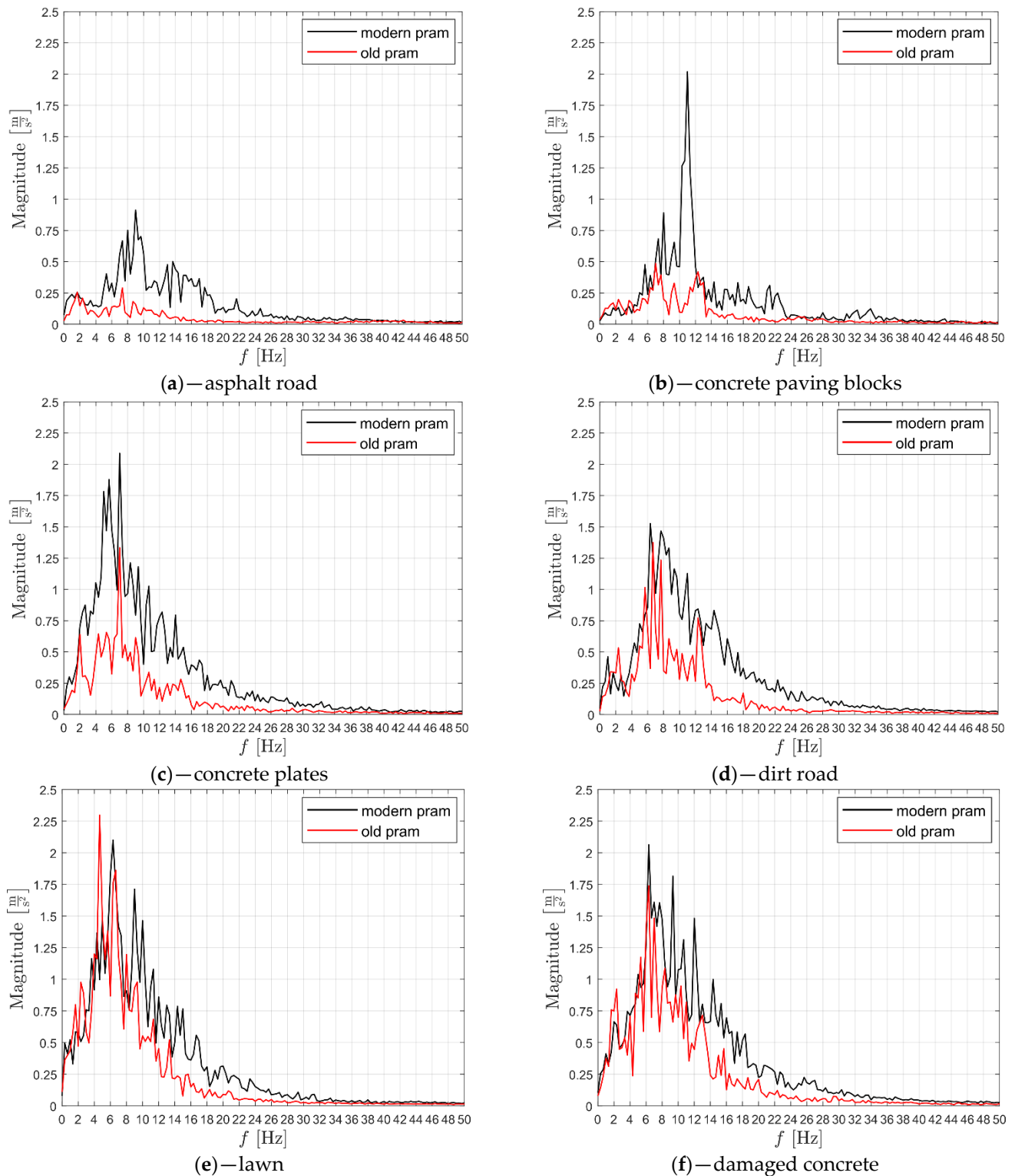
Figure 5. Amplitude-frequency spectra of vibrations of the test object within the frequency range (0, 50 Hz) when stimulated by all six considered types of surfaces.
