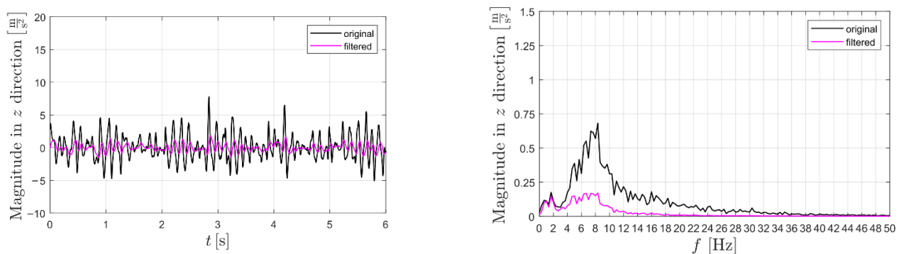
Figure 7. Comparison of vibration acceleration orthogonal components for dirt road (Figure 2d) between original (black) and frequency-weighted (purple) in both time and frequency domains.
