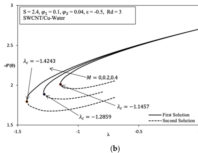
Figure 3. Variation versus \lambda with different values of M for SWCNT/Cu-water when S = 2.4 , \varphi_1 = 0.1 , \varphi_2 = 0.04 , \varepsilon = -0.5 , Gr = 0 , and Rd = 3 : (a) variation on f''(0) ; (b) variation on -\theta'(0) .
