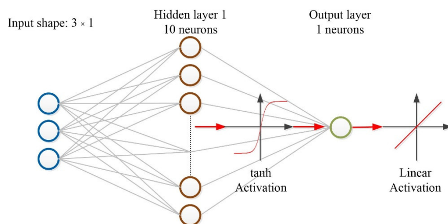
Figure 10. Architecture of the BPNN.
