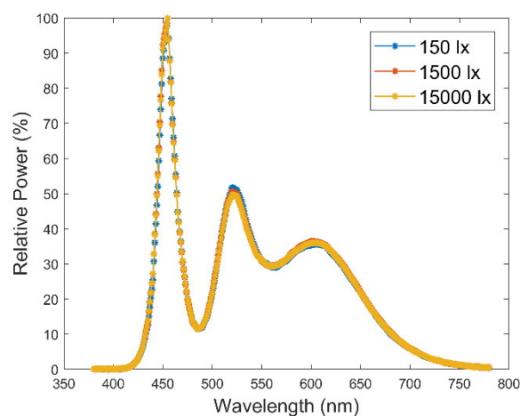
Figure 2. The spectral power distributions (SPDs) of the light sources.
