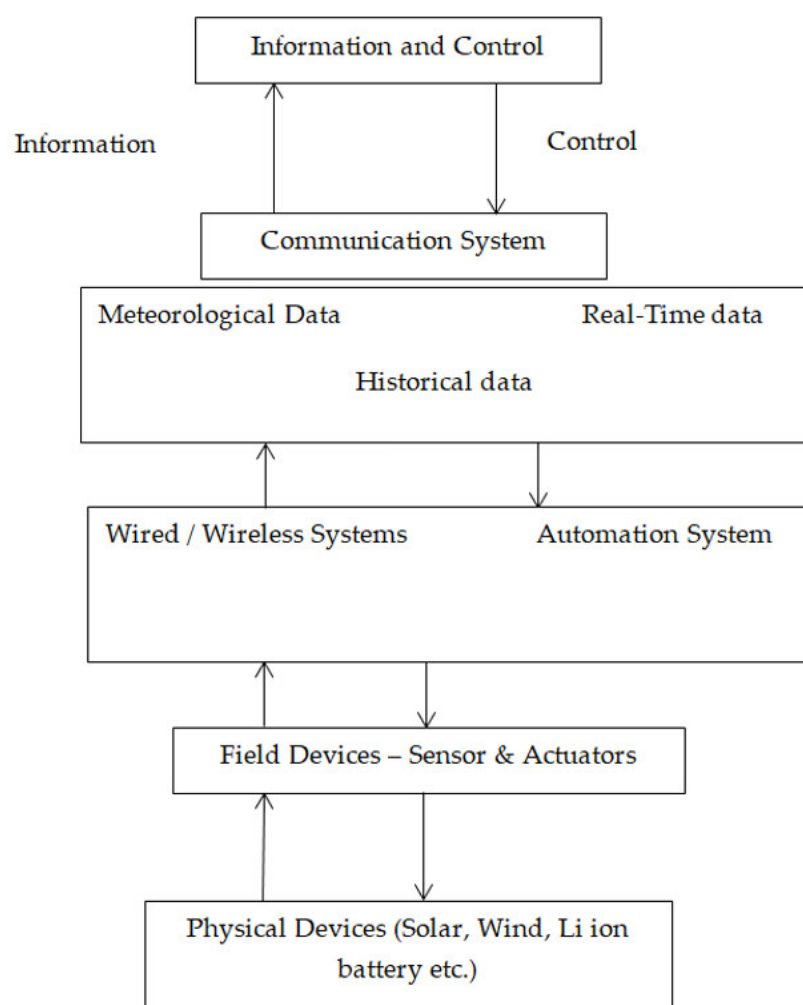
Figure 6. Typical smart microgrid with cyber secure systems.
