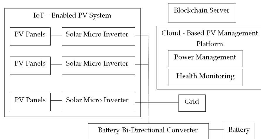
Figure 9. Architecture of IoT-enabled PV system.
