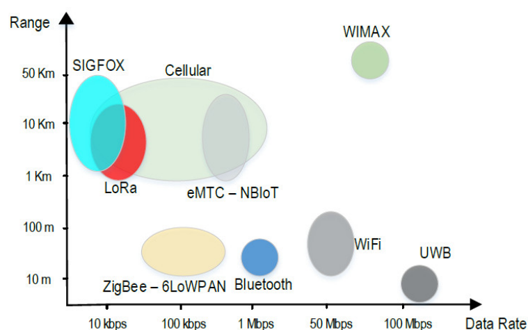
Figure 5. Comparison of different wireless topologies as a function of distance and speed.
