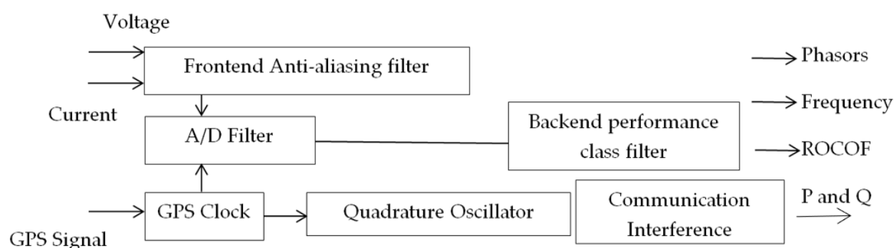
Figure 7. PMU block diagram.
