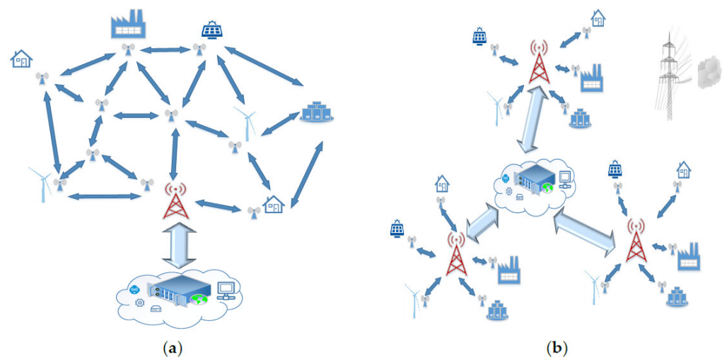
Figure 4. (a,b) shows the schematic of ZigBee (Mesh) and of LoRa (Star).
