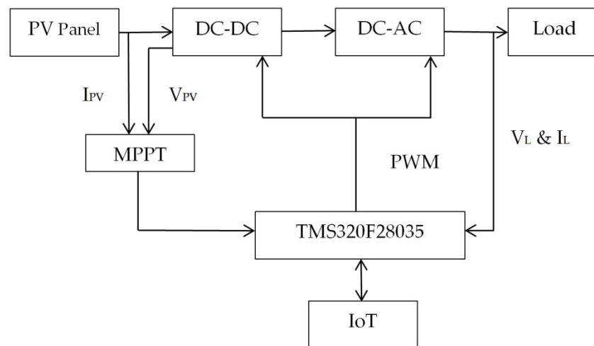
Figure 11. Topology and the control strategy of the IoT-enabled smart inverter.
