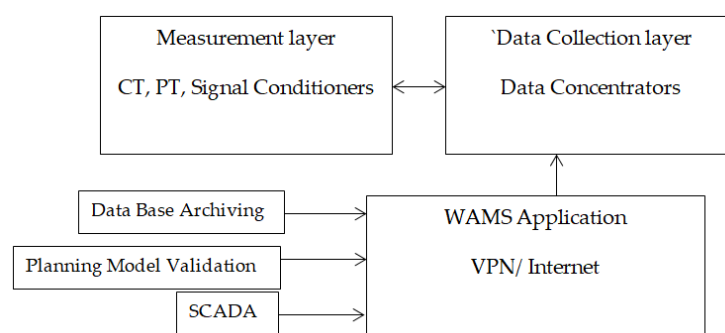
Figure 8. Basic architecture of ST.
