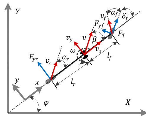
Figure 3. Vehicle dynamics model considering force coupling.
