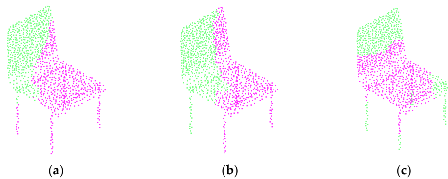
Figure 8. Accuracy of correspondence point estimation: (a) TPCC-Net, p = 0.90 ; (b) PRNet, p = 0.51 ; (c) RPM-Net, p = 0.25 .
