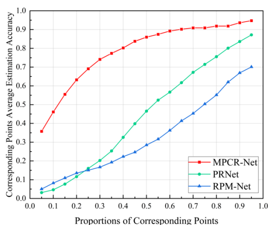
Figure 9. Average estimation accuracy of correspondence points with different proportions of correspondence points.
