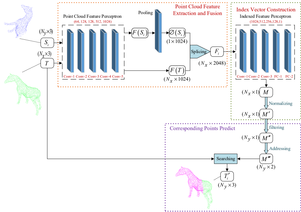
Figure 2. The network architecture of the TPCC-Net.
