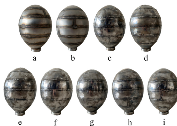
Figure 13. Photo of egg-shaped pressure hulls.
