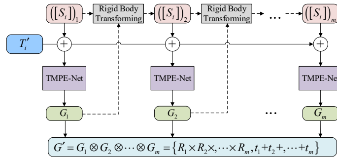
Figure 5. The iterative estimation of rigid body transformation.
