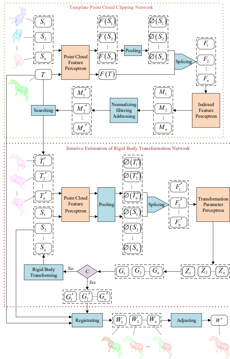
Figure 1. The network architecture of the MPCR-Net.
