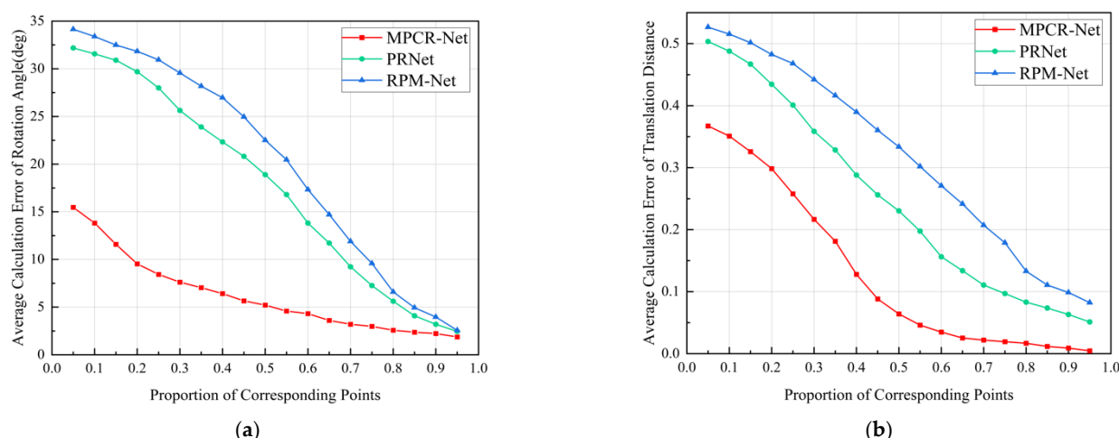
Figure 11. Average registration error with different proportions of correspondence points: (a) Average calculation error of rotation angle; (b) Average calculation error of translation distance.
