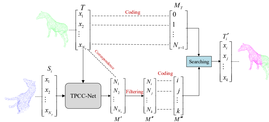
Figure 3. The estimating process of the correspondence points.
