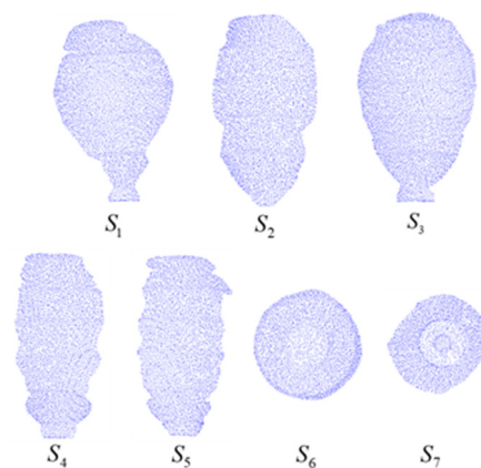
Figure 16. Partial point clouds of the hull ‘a’ at different scanning angles.
