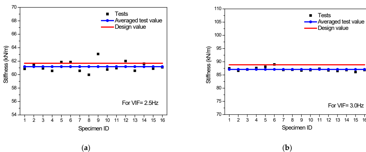
Figure 10. Comparison of stiffness between tests and design values of helical coil springs: (a) For VIF = 2.5 Hz; (b) for VIF = 3.0 Hz.
