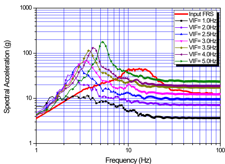
Figure 5. Spectral acceleration response of superstructure for various design VIF.
