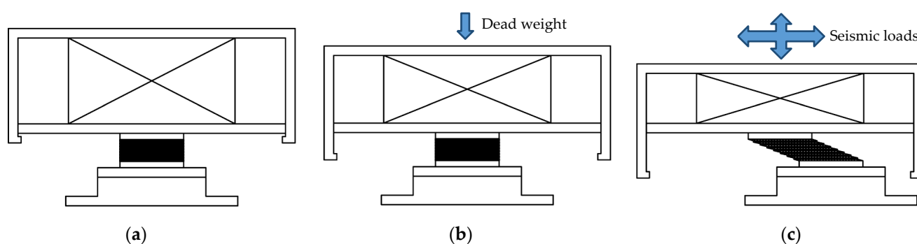
Figure 2. Schematics of 3D seismic isolator's motions: (a) Without loads; (b) with vertical static load; (c) with horizontal and vertical seismic loads.
