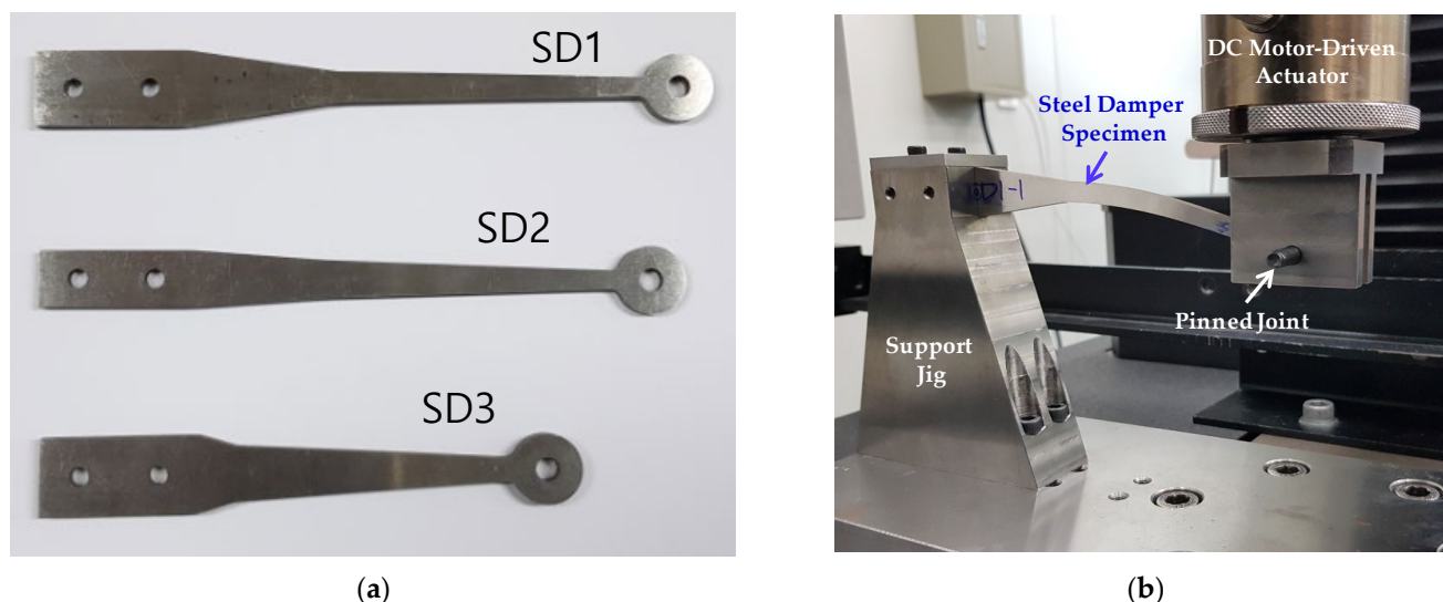
Figure 16. Photos of steel damper specimen and test facility: (a) Steel damper specimen; (b) test facility with specimen.
