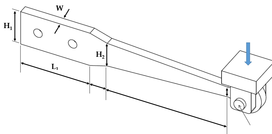
Figure 11. Configurations and dimensional parameters of steel damper.
