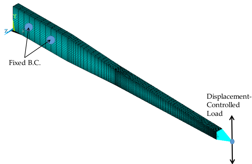
Figure 12. Finite element model of steel damper for energy dissipation analysis.
