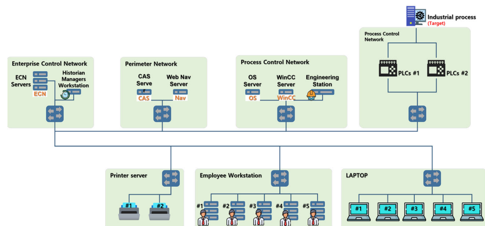
Figure 11. STUXNET case-based network topology (Physical).
