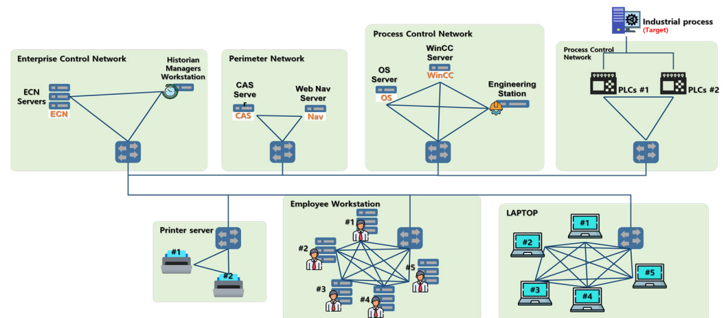
Figure 12. STUXNET case-based network topology (Logical).
