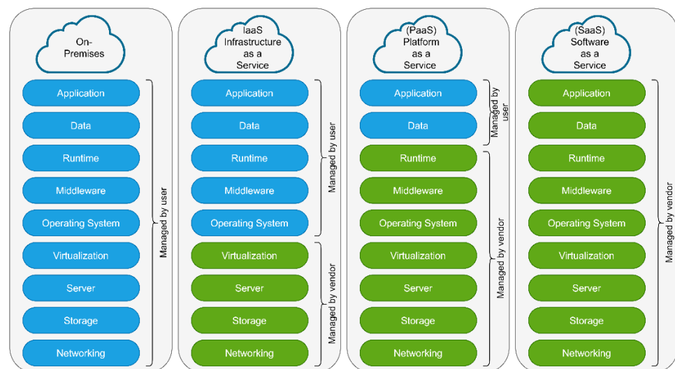
Figure 1. IaaS-PaaS-SaaS comparison [4].
