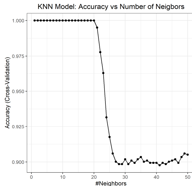
Figure 6. KNN model accuracy versus the number of neighbours.
