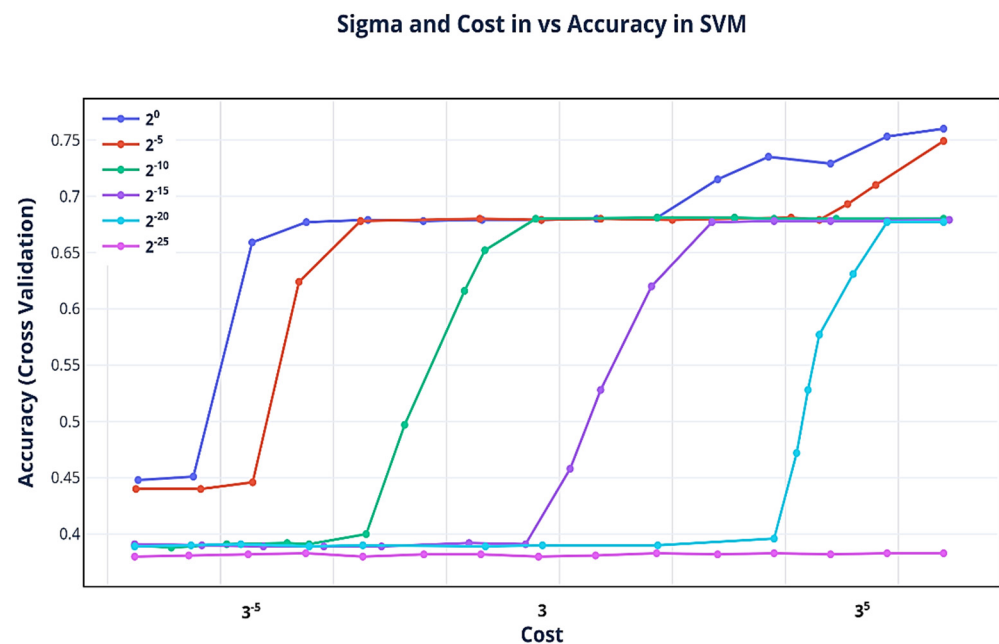
Figure 9. SVM model accuracy for various sigma and cost values.
