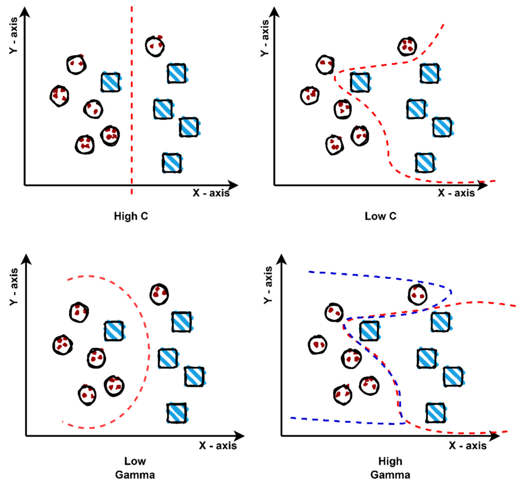
Figure 5. The effect of the SVM parameter setting on the hyperplane.
