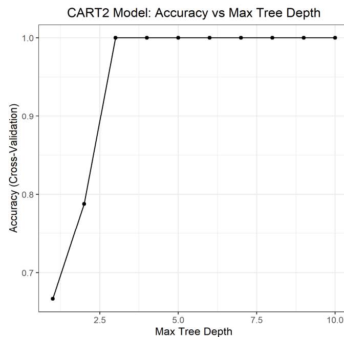
Figure 7. CART model accuracy versus max tree depth.
