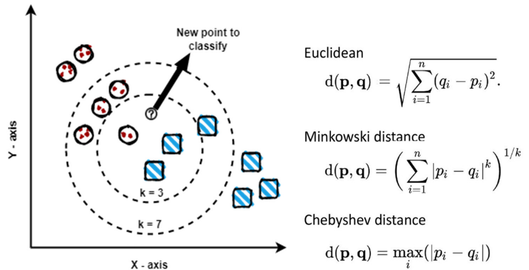
Figure 2. KNN model calculation and technique visualisation.
