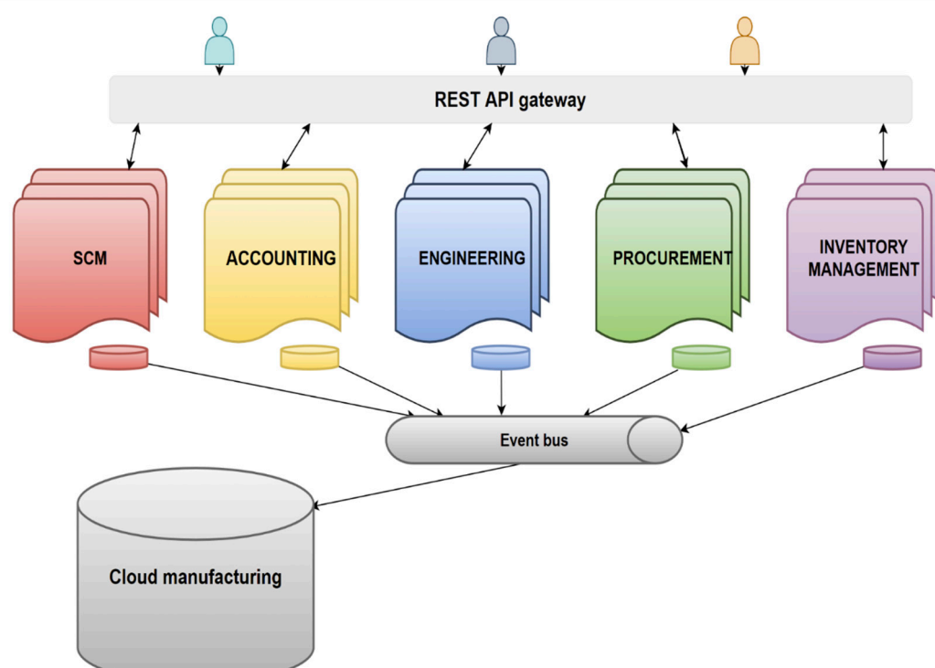
Figure 5. BCaaS and SCM system architecture for boxed sheet metal manufacturing.
