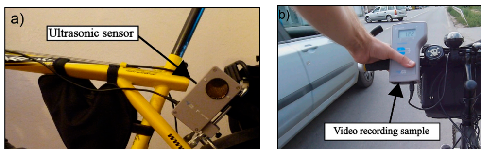
Figure 1. Presentation of the ultrasonic sensor used in the experiment (a) and an example of the video recording (b).
