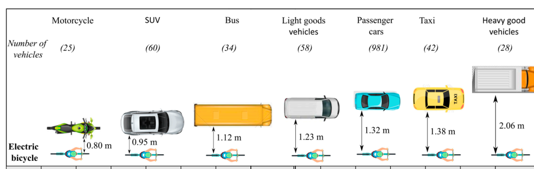
Figure 4. Average lateral distance when overtaking an e-bicycle according to vehicle categories.
