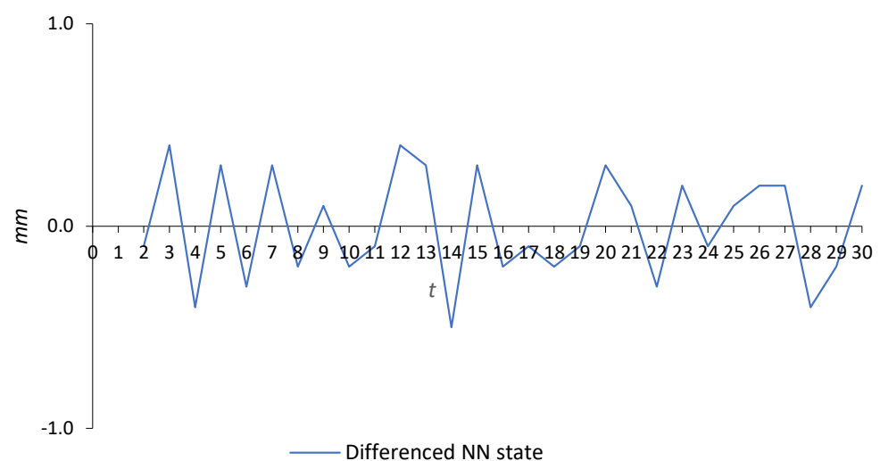
Figure 7. Stationary series.
