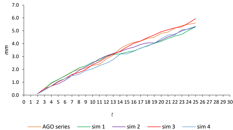
Figure 10. Four simulations of AGO series.
