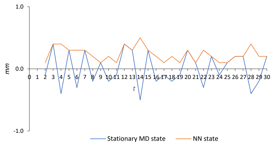
Figure 8. Transformation of stationary MD state of series.
