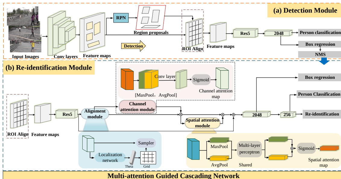
Figure 2. The flow chart of a Multi-Attention-Guided Cascading Network (MGCN), which integrates multi-attention discriminative information from a person in an end-to-end network for person search task. MGCN first mark multiple person by detection network, which provides a high-quality bounding box for each person to obtain label information. Then, MGCN utilize aligning module to locate advanced semantic information from the input image and avoid interference caused by background information. Finally, we introduce a multi-attention module to promote network focus on distinguishing fine-grained information between the multiple person for the re-id task.
