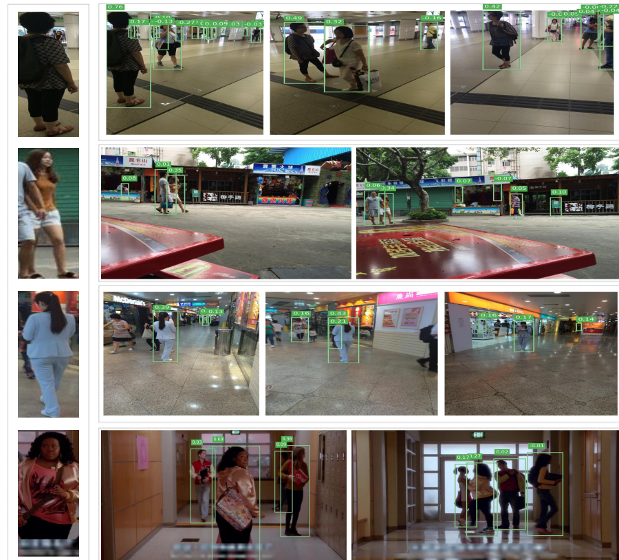
Figure 6. Visualization results of person search. The left side represents pedestrians to be detected and the green bounding boxes represent search results with different probabilities.
