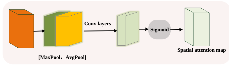
Figure 5. Spatial attention model.
