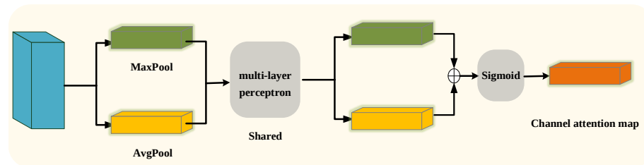
Figure 4. Channel attention model.
