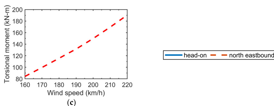
Figure 11. Internal forces determined in the column base of the billboard for head-on and north eastbound wind speed directions across the adopted wind speeds: (a) base shear force; (b) bending moment and (c) torsional moment.
