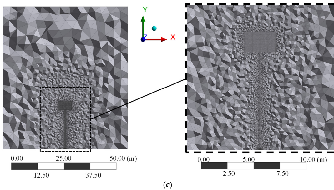
Figure 6. CFD model: (a) air volume, boundary conditions, geometry of the billboard and wind directions; (b) longitudinal section; (c) cross section.
